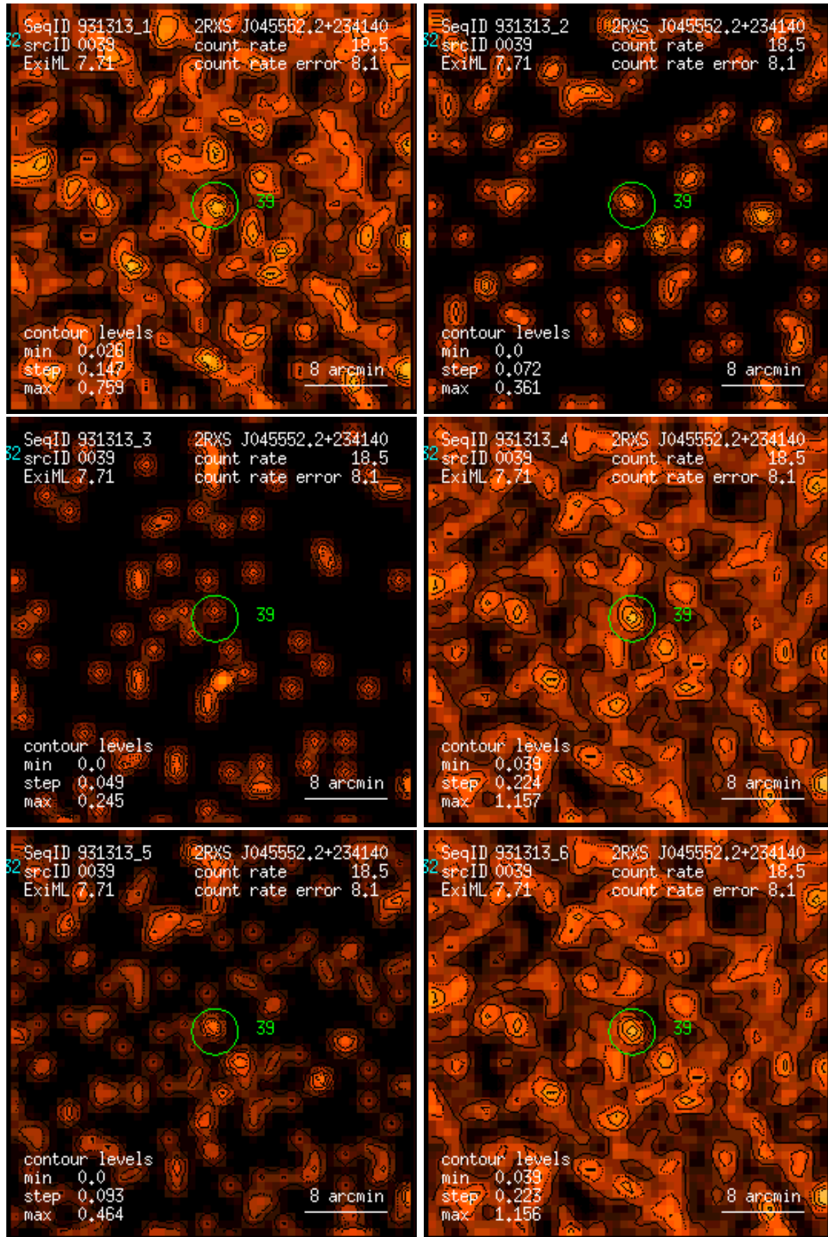
Figure 39: RASS 931313: detection 0039: band rate images, Gaussian filter: (1) PSPC channels 11 – 41, (2) 52 – 90, (3) 91 – 201, (4) 11 – 235, (5) 52 – 201, (6) 11 – 201. Broad band rates in counts/ks. Band rate contour levels in counts/ks/arcmin 2 .
