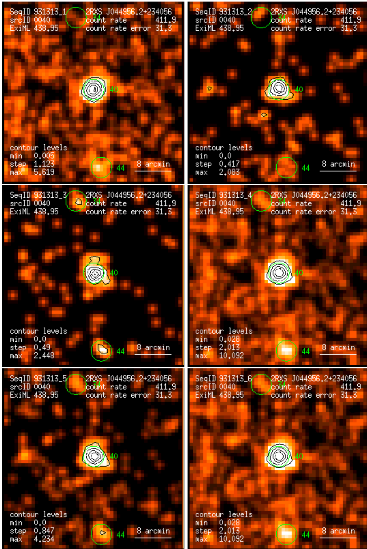
Figure 40: RASS 931313: detection 0040: band rate images, Gaussian filter: (1) PSPC channels 11 – 41, (2) 52 – 90, (3) 91 – 201, (4) 11 – 235, (5) 52 – 201, (6) 11 – 201. Broad band rates in counts/ks. Band rate contour levels in counts/ks/arcmin 2 .
