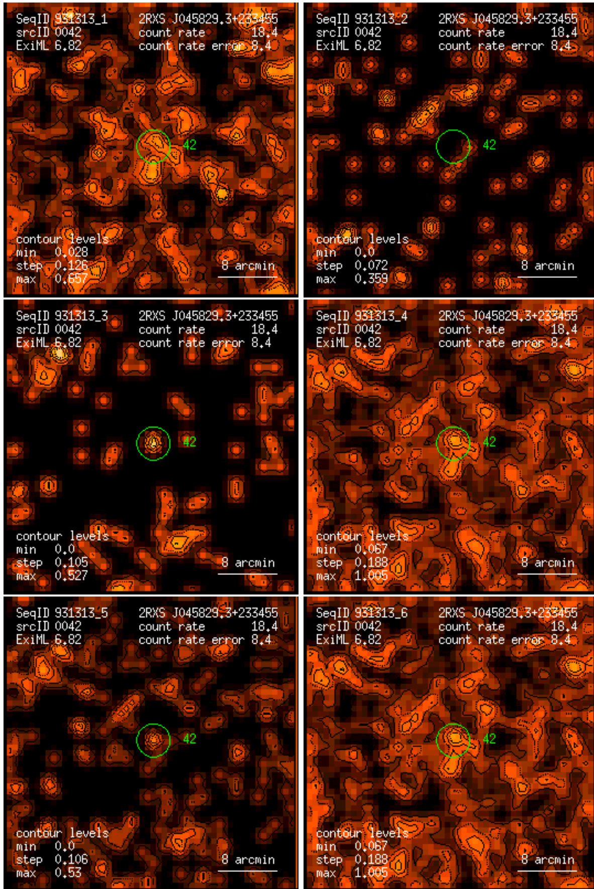
Figure 42: RASS 931313: detection 0042: band rate images, Gaussian filter: (1) PSPC channels 11 – 41, (2) 52 – 90, (3) 91 – 201, (4) 11 – 235, (5) 52 – 201, (6) 11 – 201. Broad band rates in counts/ks. Band rate contour levels in counts/ks/arcmin 2 .
