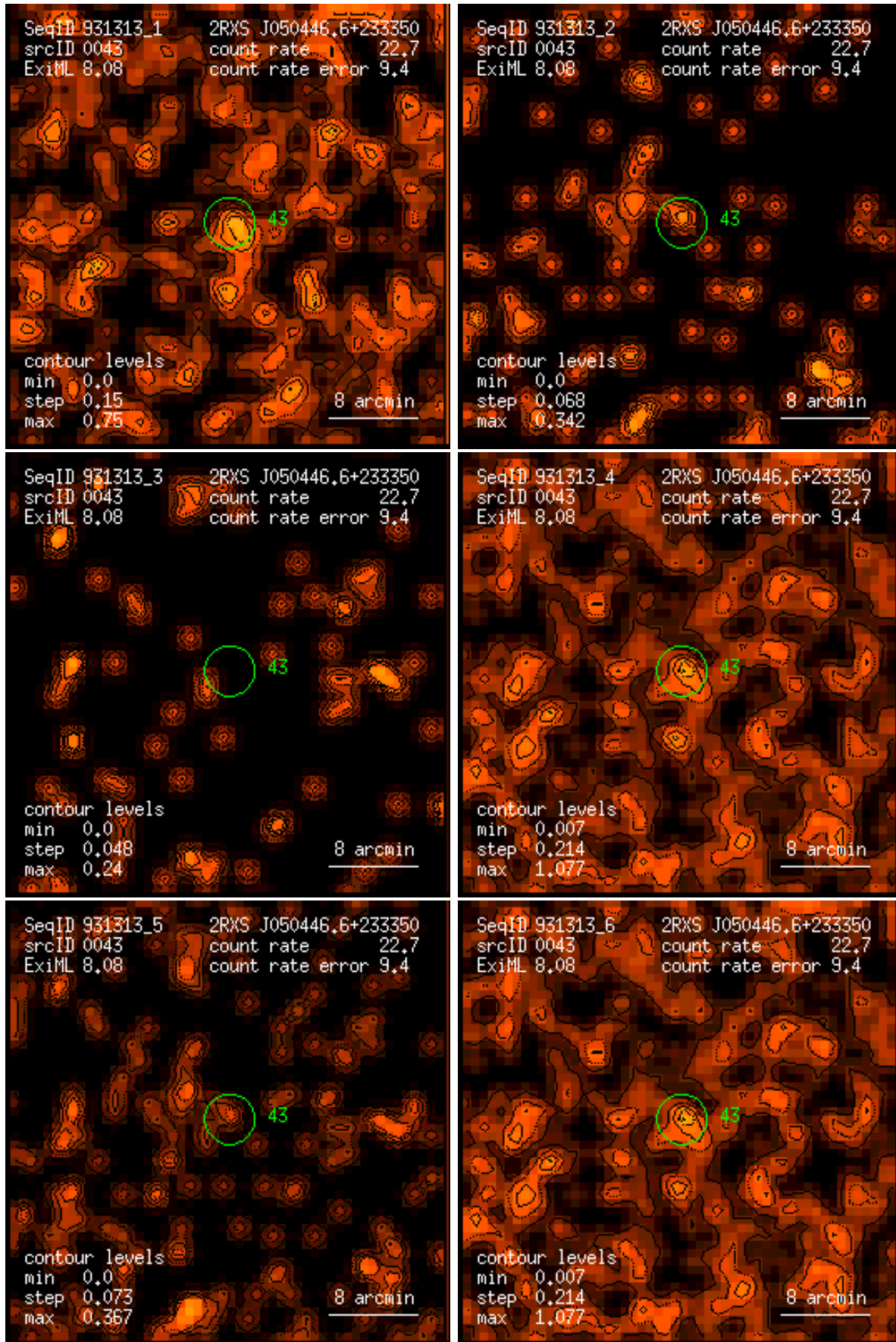
Figure 43: RASS 931313: detection 0043: band rate images, Gaussian filter: (1) PSPC channels 11 – 41, (2) 52 – 90, (3) 91 – 201, (4) 11 – 235, (5) 52 – 201, (6) 11 – 201. Broad band rates in counts/ks. Band rate contour levels in counts/ks/arcmin 2 .
