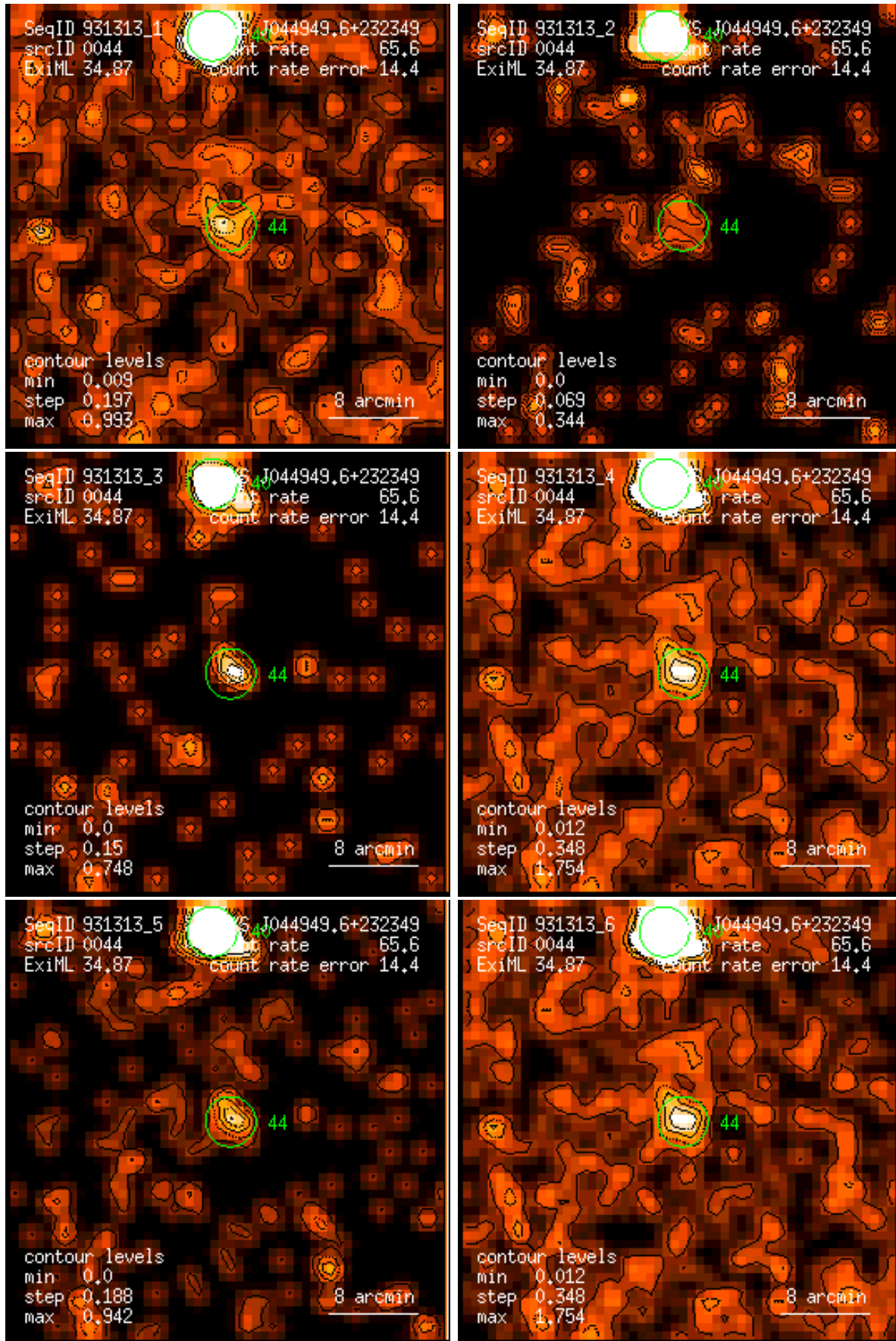
Figure 44: RASS 931313: detection 0044: band rate images, Gaussian filter: (1) PSPC channels 11 – 41, (2) 52 – 90, (3) 91 – 201, (4) 11 – 235, (5) 52 – 201, (6) 11 – 201. Broad band rates in counts/ks. Band rate contour levels in counts/ks/arcmin 2 .
