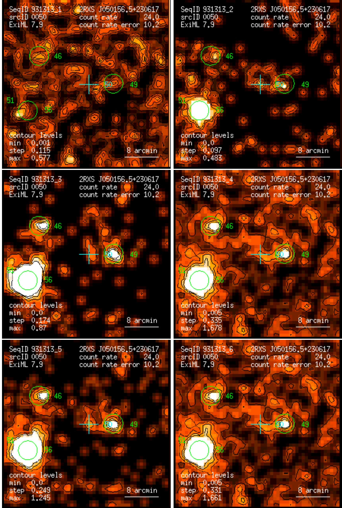
Figure 50: RASS 931313: detection 0050: band rate images, Gaussian filter: (1) PSPC channels 11 – 41, (2) 52 – 90, (3) 91 – 201, (4) 11 – 235, (5) 52 – 201, (6) 11 – 201. Broad band rates in counts/ks. Band rate contour levels in counts/ks/arcmin 2 .
