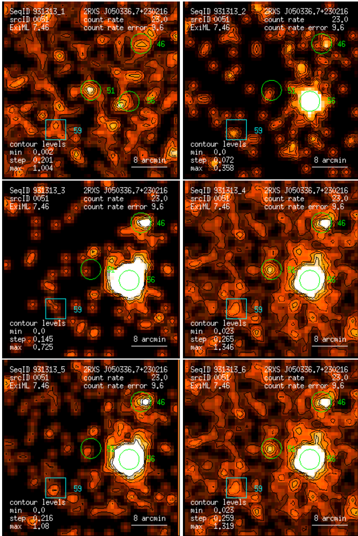
Figure 51: RASS 931313: detection 0051: band rate images, Gaussian filter: (1) PSPC channels 11 – 41, (2) 52 – 90, (3) 91 – 201, (4) 11 – 235, (5) 52 – 201, (6) 11 – 201. Broad band rates in counts/ks. Band rate contour levels in counts/ks/arcmin 2 .
