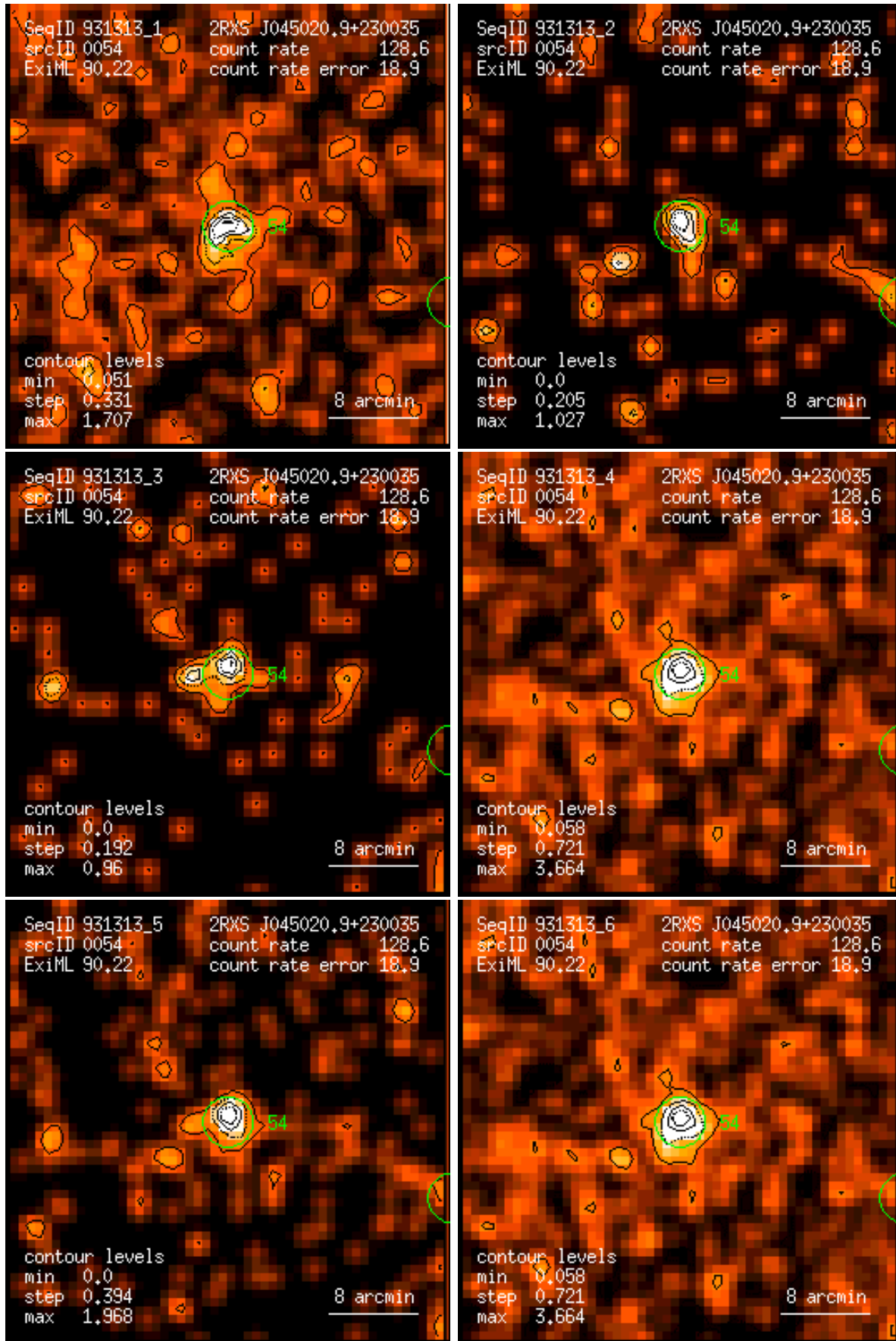
Figure 54: RASS 931313: detection 0054: band rate images, Gaussian filter: (1) PSPC channels 11 – 41, (2) 52 – 90, (3) 91 – 201, (4) 11 – 235, (5) 52 – 201, (6) 11 – 201. Broad band rates in counts/ks. Band rate contour levels in counts/ks/arcmin 2 .
