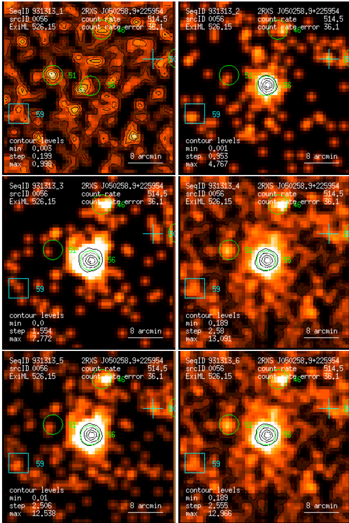
Figure 56: RASS 931313: detection 0056: band rate images, Gaussian filter: (1) PSPC channels 11 – 41, (2) 52 – 90, (3) 91 – 201, (4) 11 – 235, (5) 52 – 201, (6) 11 – 201. Broad band rates in counts/ks. Band rate contour levels in counts/ks/arcmin 2 .
