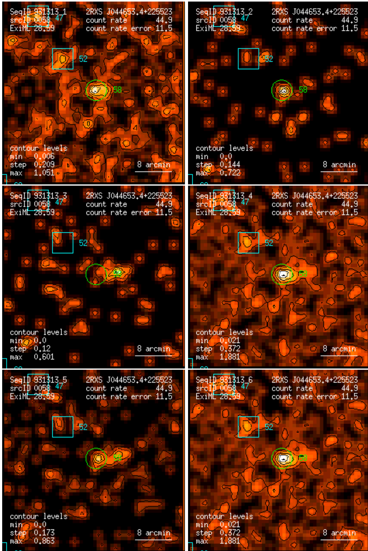
Figure 58: RASS 931313: detection 0058: band rate images, Gaussian filter: (1) PSPC channels 11 – 41, (2) 52 – 90, (3) 91 – 201, (4) 11 – 235, (5) 52 – 201, (6) 11 – 201. Broad band rates in counts/ks. Band rate contour levels in counts/ks/arcmin 2 .
