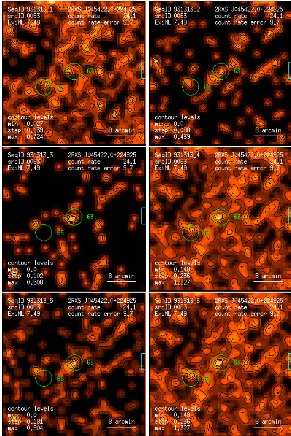
Figure 63: RASS 931313: detection 0063: band rate images, Gaussian filter: (1) PSPC channels 11 – 41, (2) 52 – 90, (3) 91 – 201, (4) 11 – 235, (5) 52 – 201, (6) 11 – 201. Broad band rates in counts/ks. Band rate contour levels in counts/ks/arcmin 2 .
