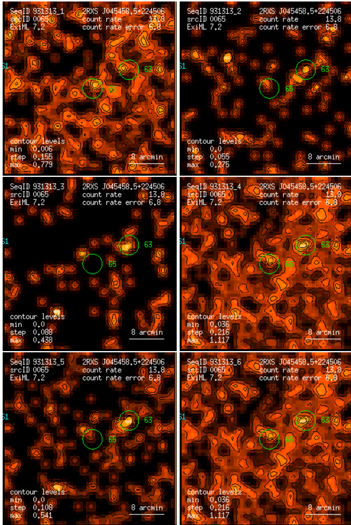
Figure 65: RASS 931313: detection 0065: band rate images, Gaussian filter: (1) PSPC channels 11 – 41, (2) 52 – 90, (3) 91 – 201, (4) 11 – 235, (5) 52 – 201, (6) 11 – 201. Broad band rates in counts/ks. Band rate contour levels in counts/ks/arcmin 2 .
