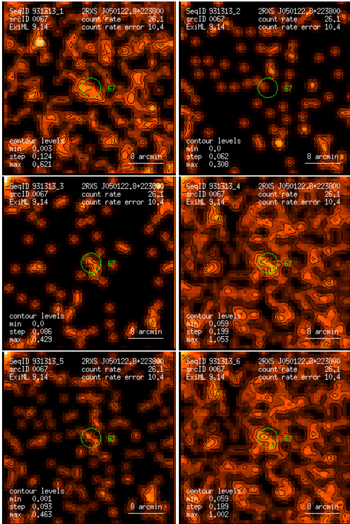
Figure 67: RASS 931313: detection 0067: band rate images, Gaussian filter: (1) PSPC channels 11 – 41, (2) 52 – 90, (3) 91 – 201, (4) 11 – 235, (5) 52 – 201, (6) 11 – 201. Broad band rates in counts/ks. Band rate contour levels in counts/ks/arcmin 2 .
