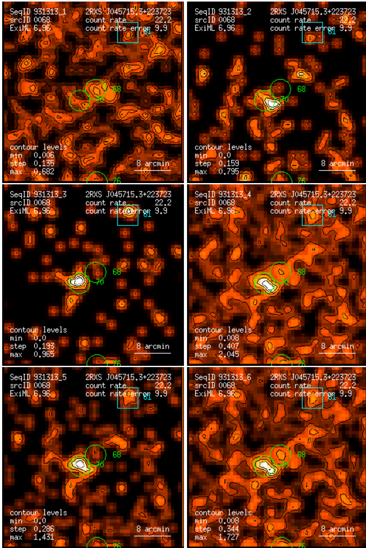
Figure 68: RASS 931313: detection 0068: band rate images, Gaussian filter: (1) PSPC channels 11 – 41, (2) 52 – 90, (3) 91 – 201, (4) 11 – 235, (5) 52 – 201, (6) 11 – 201. Broad band rates in counts/ks. Band rate contour levels in counts/ks/arcmin 2 .
