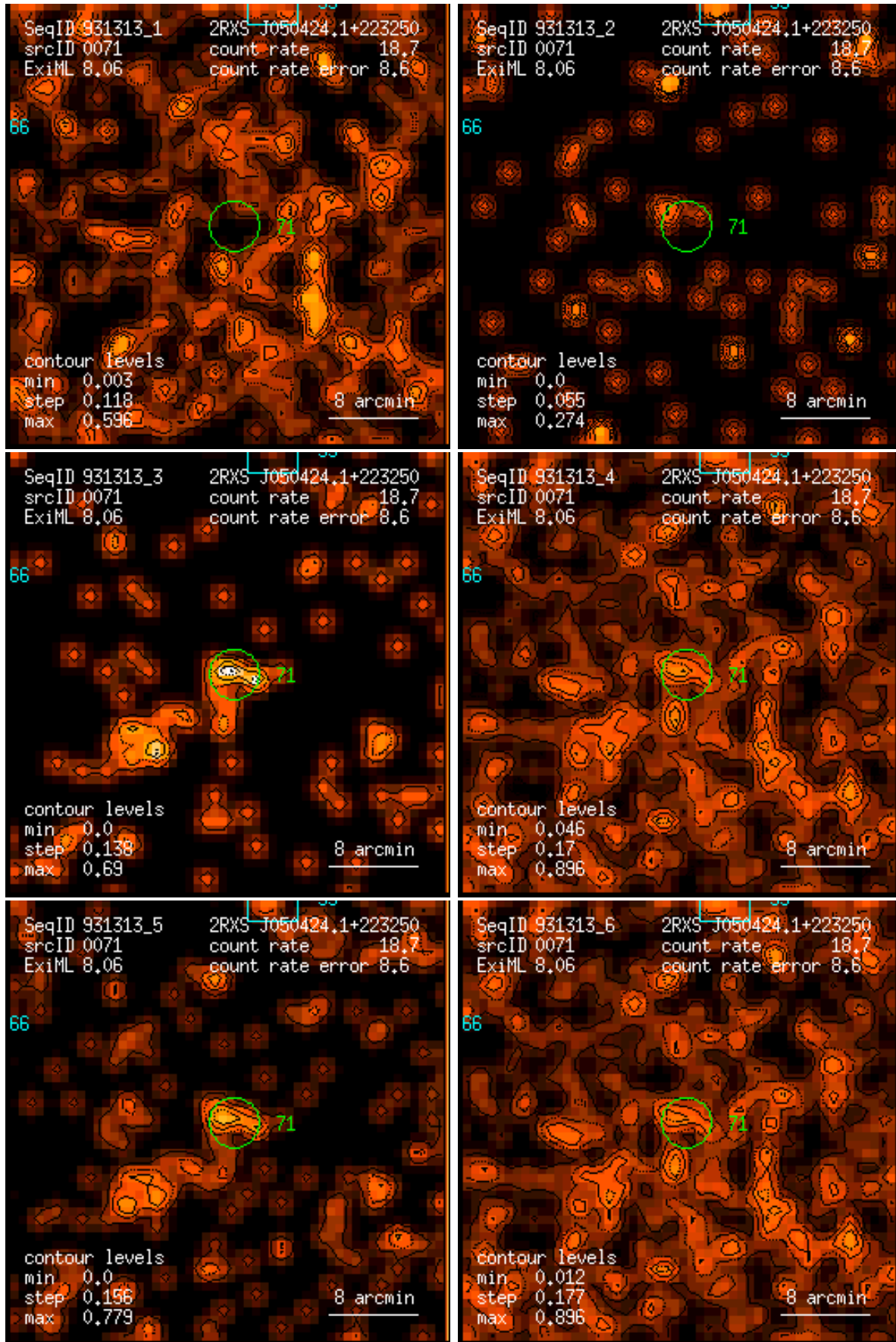
Figure 71: RASS 931313: detection 0071: band rate images, Gaussian filter: (1) PSPC channels 11 – 41, (2) 52 – 90, (3) 91 – 201, (4) 11 – 235, (5) 52 – 201, (6) 11 – 201. Broad band rates in counts/ks. Band rate contour levels in counts/ks/arcmin 2 .
