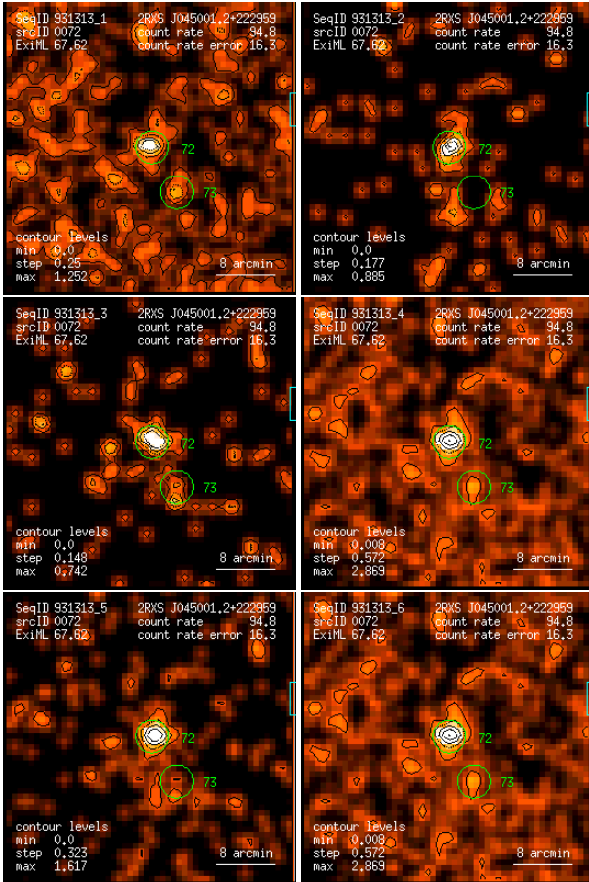
Figure 72: RASS 931313: detection 0072: band rate images, Gaussian filter: (1) PSPC channels 11 – 41, (2) 52 – 90, (3) 91 – 201, (4) 11 – 235, (5) 52 – 201, (6) 11 – 201. Broad band rates in counts/ks. Band rate contour levels in counts/ks/arcmin 2 .
