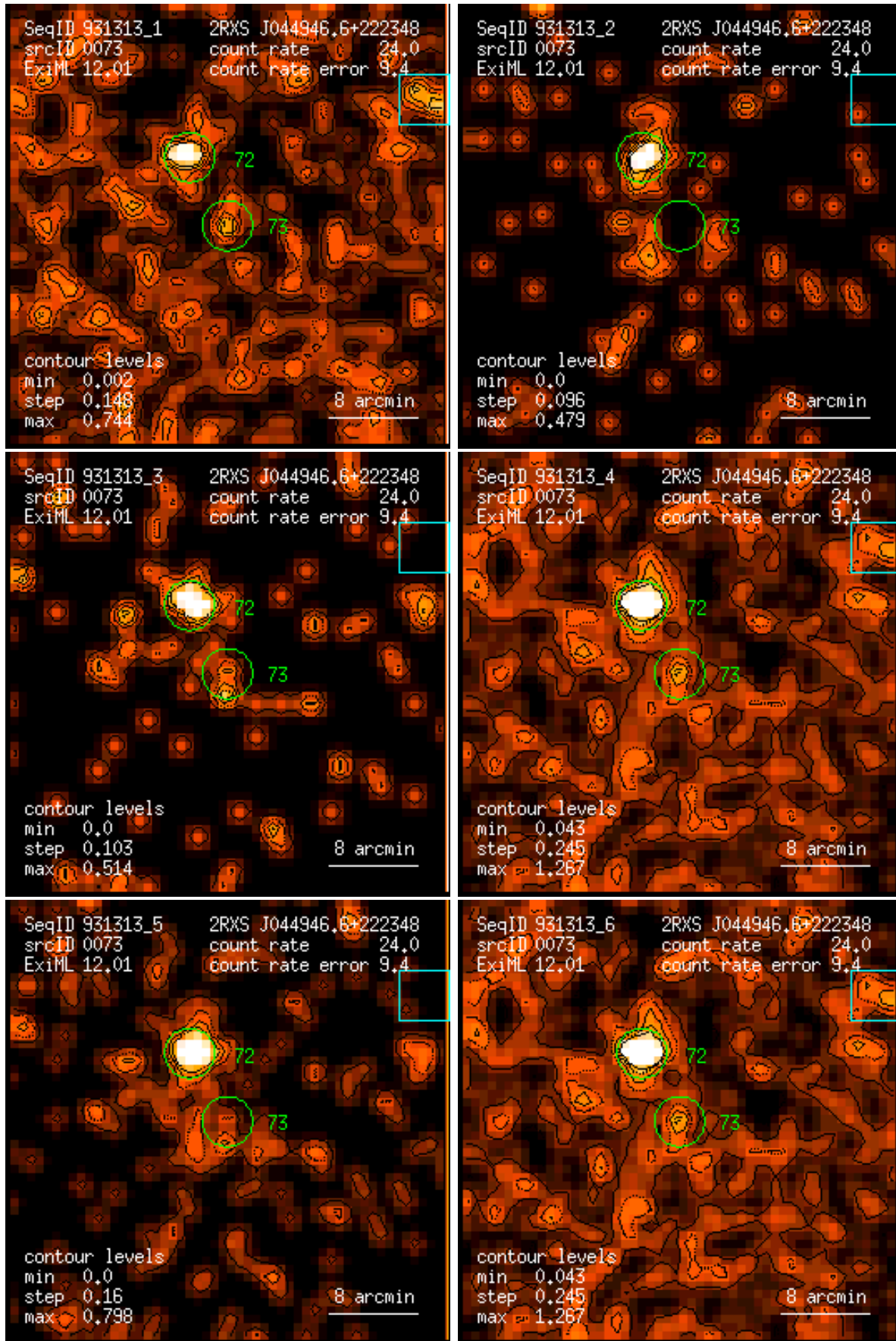
Figure 73: RASS 931313: detection 0073: band rate images, Gaussian filter: (1) PSPC channels 11 – 41, (2) 52 – 90, (3) 91 – 201, (4) 11 – 235, (5) 52 – 201, (6) 11 – 201. Broad band rates in counts/ks. Band rate contour levels in counts/ks/arcmin 2 .
