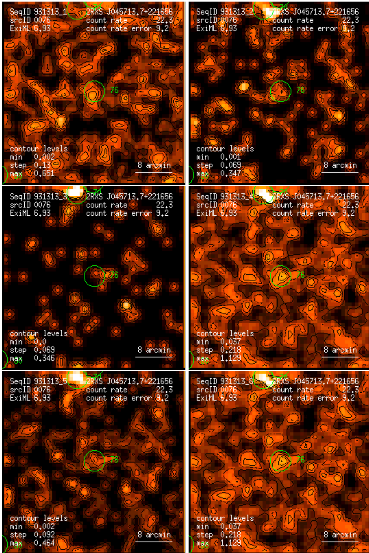
Figure 76: RASS 931313: detection 0076: band rate images, Gaussian filter: (1) PSPC channels 11 – 41, (2) 52 – 90, (3) 91 – 201, (4) 11 – 235, (5) 52 – 201, (6) 11 – 201. Broad band rates in counts/ks. Band rate contour levels in counts/ks/arcmin 2 .
