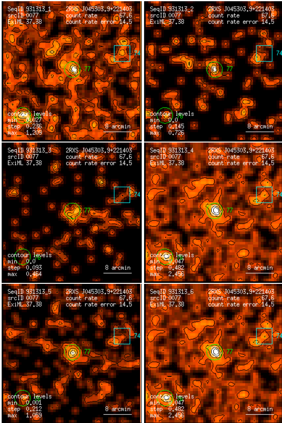
Figure 77: RASS 931313: detection 0077: band rate images, Gaussian filter: (1) PSPC channels 11 – 41, (2) 52 – 90, (3) 91 – 201, (4) 11 – 235, (5) 52 – 201, (6) 11 – 201. Broad band rates in counts/ks. Band rate contour levels in counts/ks/arcmin 2 .
