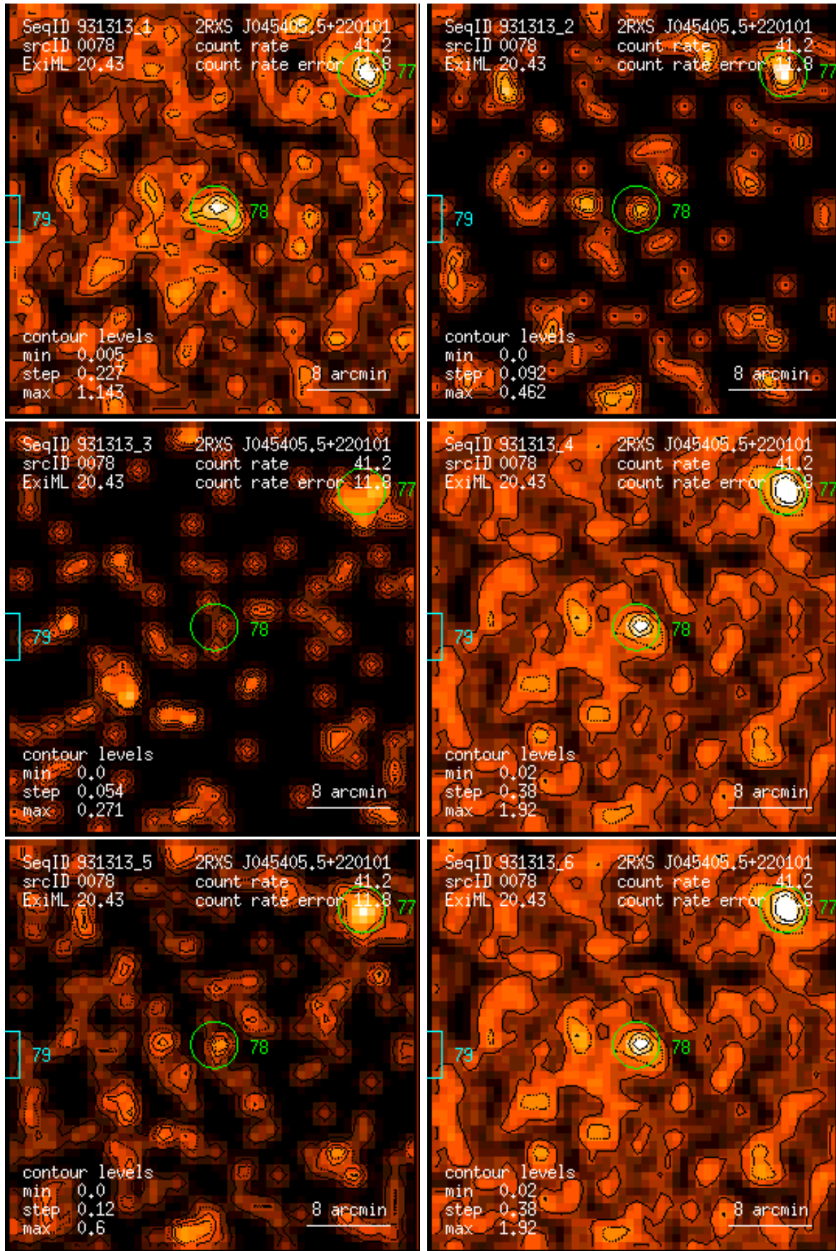
Figure 78: RASS 931313: detection 0078: band rate images, Gaussian filter: (1) PSPC channels 11 – 41, (2) 52 – 90, (3) 91 – 201, (4) 11 – 235, (5) 52 – 201, (6) 11 – 201. Broad band rates in counts/ks. Band rate contour levels in counts/ks/arcmin 2 .
