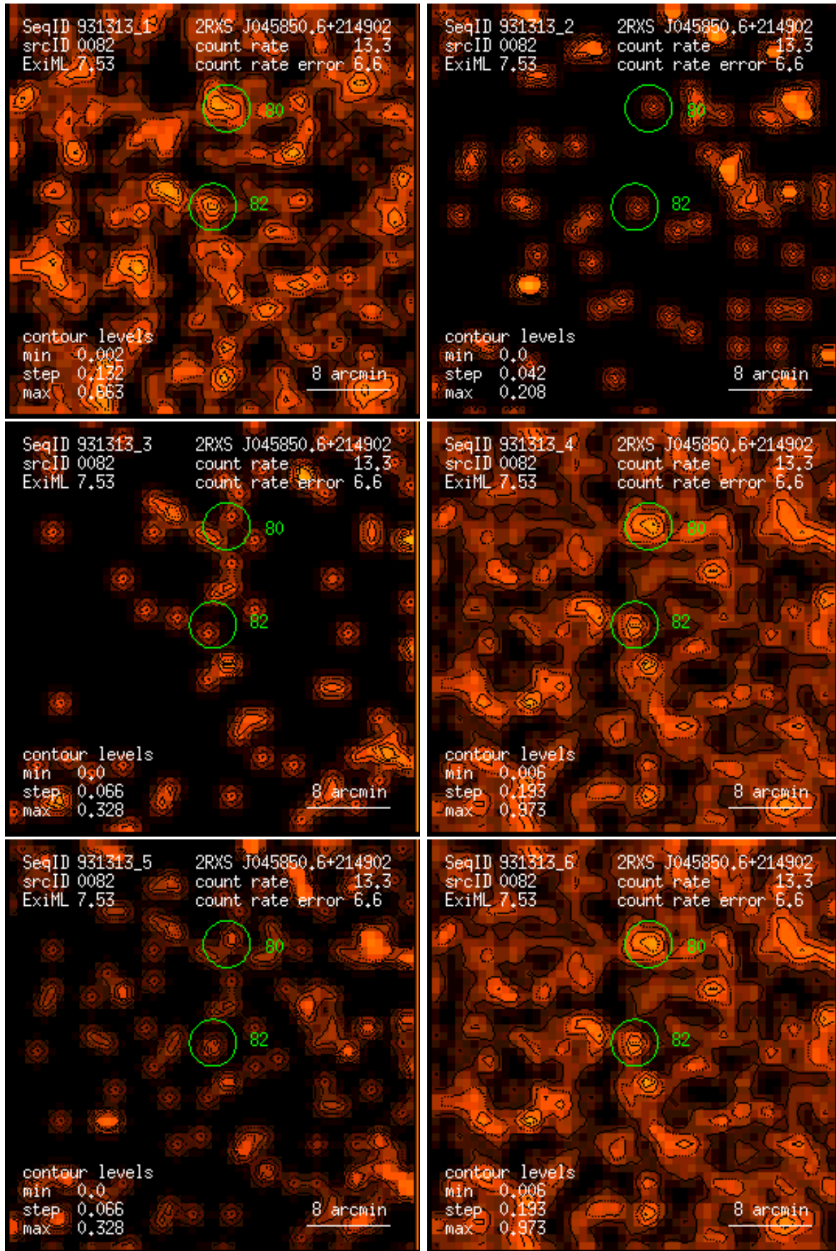
Figure 82: RASS 931313: detection 0082: band rate images, Gaussian filter: (1) PSPC channels 11 – 41, (2) 52 – 90, (3) 91 – 201, (4) 11 – 235, (5) 52 – 201, (6) 11 – 201. Broad band rates in counts/ks. Band rate contour levels in counts/ks/arcmin 2 .
