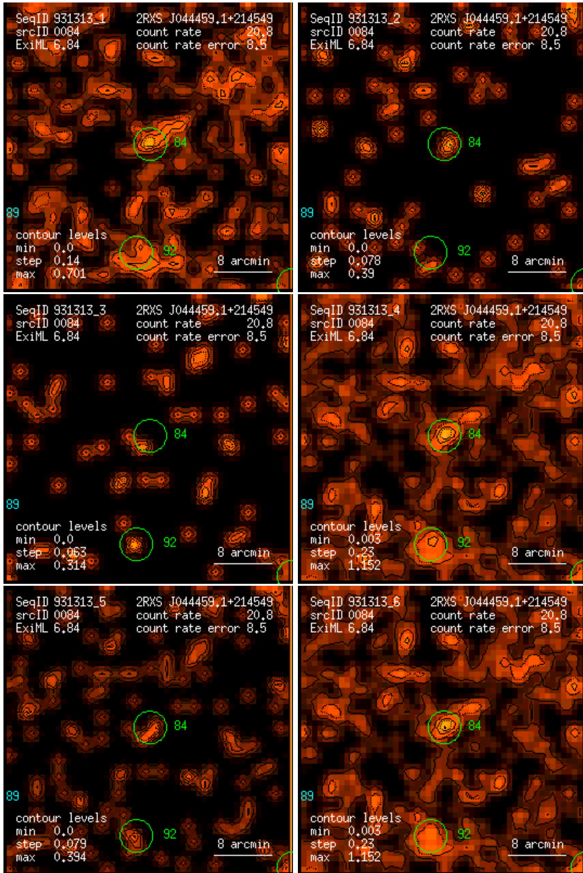
Figure 84: RASS 931313: detection 0084: band rate images, Gaussian filter: (1) PSPC channels 11 – 41, (2) 52 – 90, (3) 91 – 201, (4) 11 – 235, (5) 52 – 201, (6) 11 – 201. Broad band rates in counts/ks. Band rate contour levels in counts/ks/arcmin 2 .
