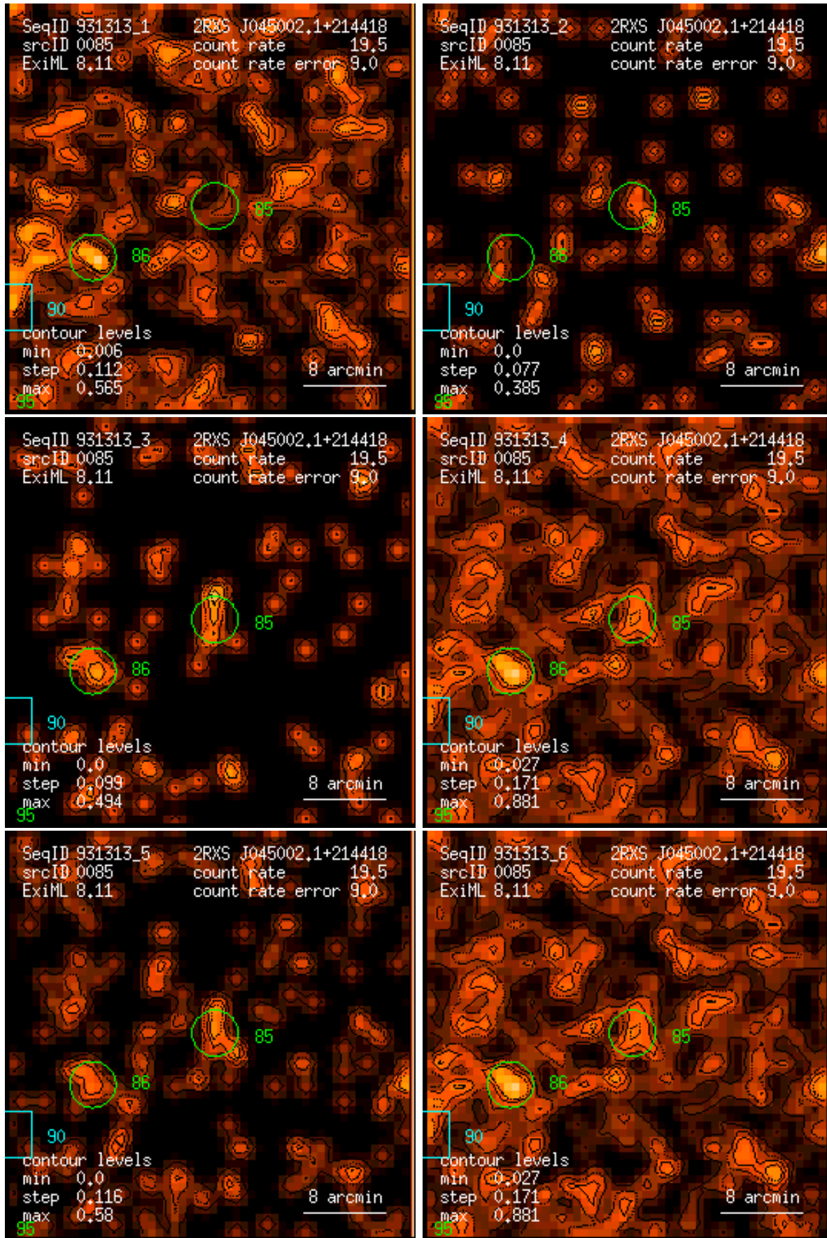
Figure 85: RASS 931313: detection 0085: band rate images, Gaussian filter: (1) PSPC channels 11 – 41, (2) 52 – 90, (3) 91 – 201, (4) 11 – 235, (5) 52 – 201, (6) 11 – 201. Broad band rates in counts/ks. Band rate contour levels in counts/ks/arcmin 2 .
