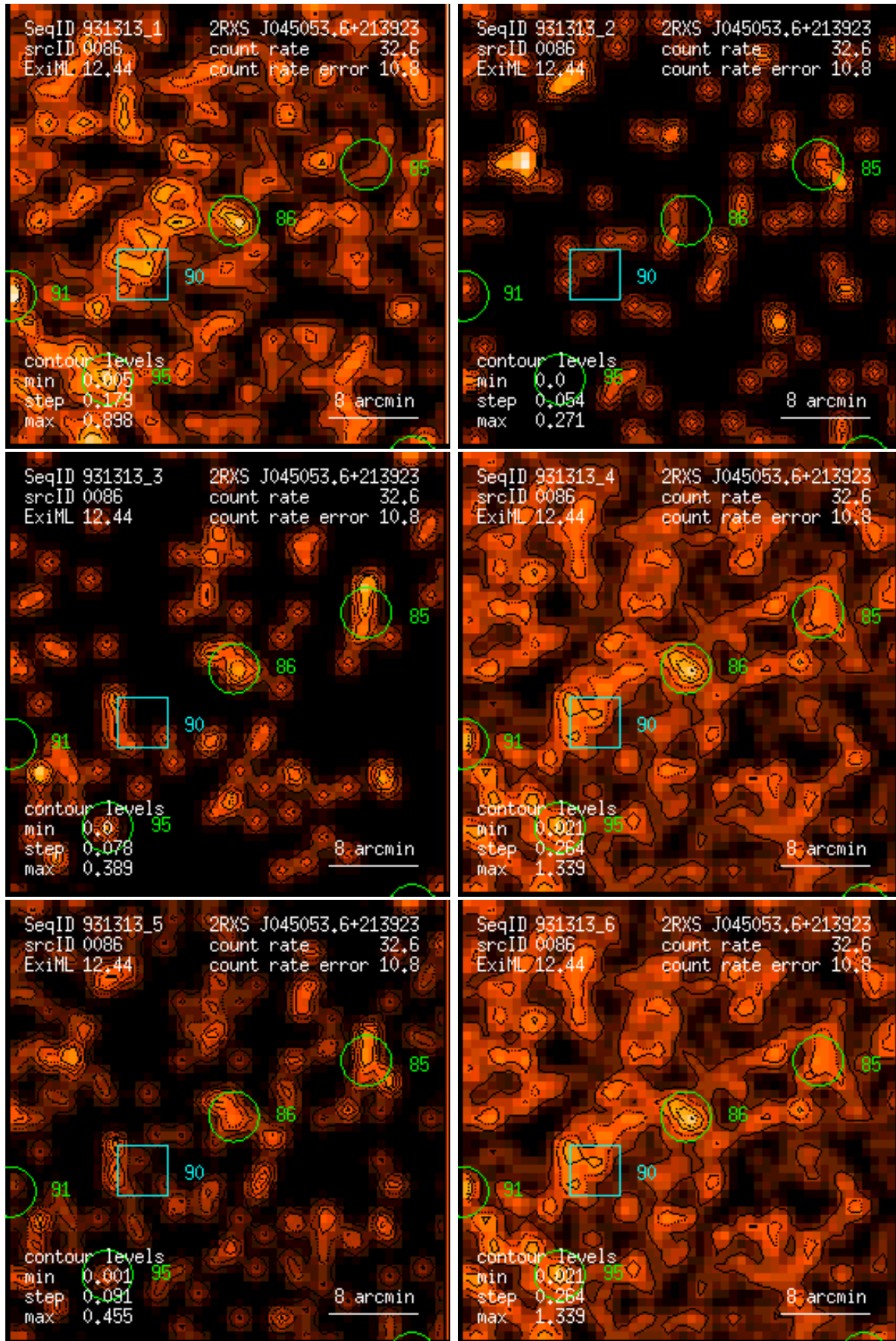
Figure 86: RASS 931313: detection 0086: band rate images, Gaussian filter: (1) PSPC channels 11 – 41, (2) 52 – 90, (3) 91 – 201, (4) 11 – 235, (5) 52 – 201, (6) 11 – 201. Broad band rates in counts/ks. Band rate contour levels in counts/ks/arcmin 2 .
