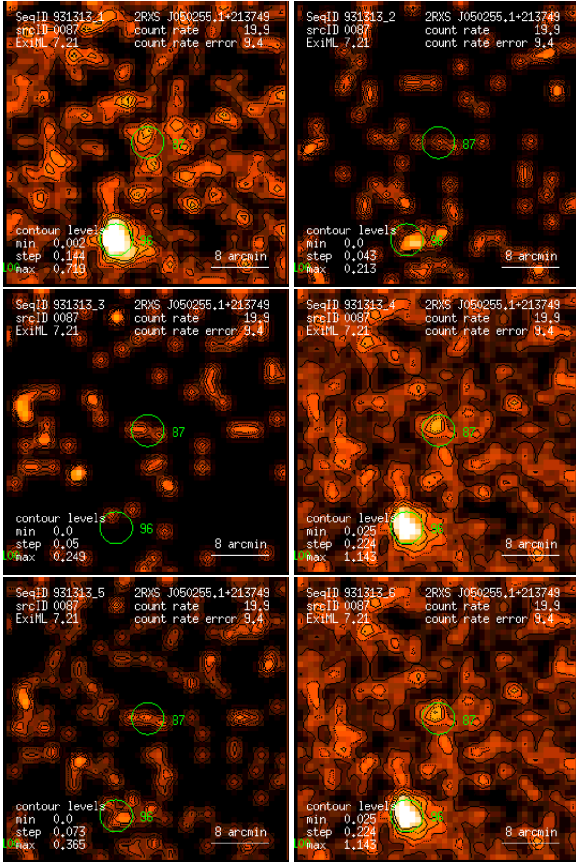
Figure 87: RASS 931313: detection 0087: band rate images, Gaussian filter: (1) PSPC channels 11 – 41, (2) 52 – 90, (3) 91 – 201, (4) 11 – 235, (5) 52 – 201, (6) 11 – 201. Broad band rates in counts/ks. Band rate contour levels in counts/ks/arcmin 2 .
