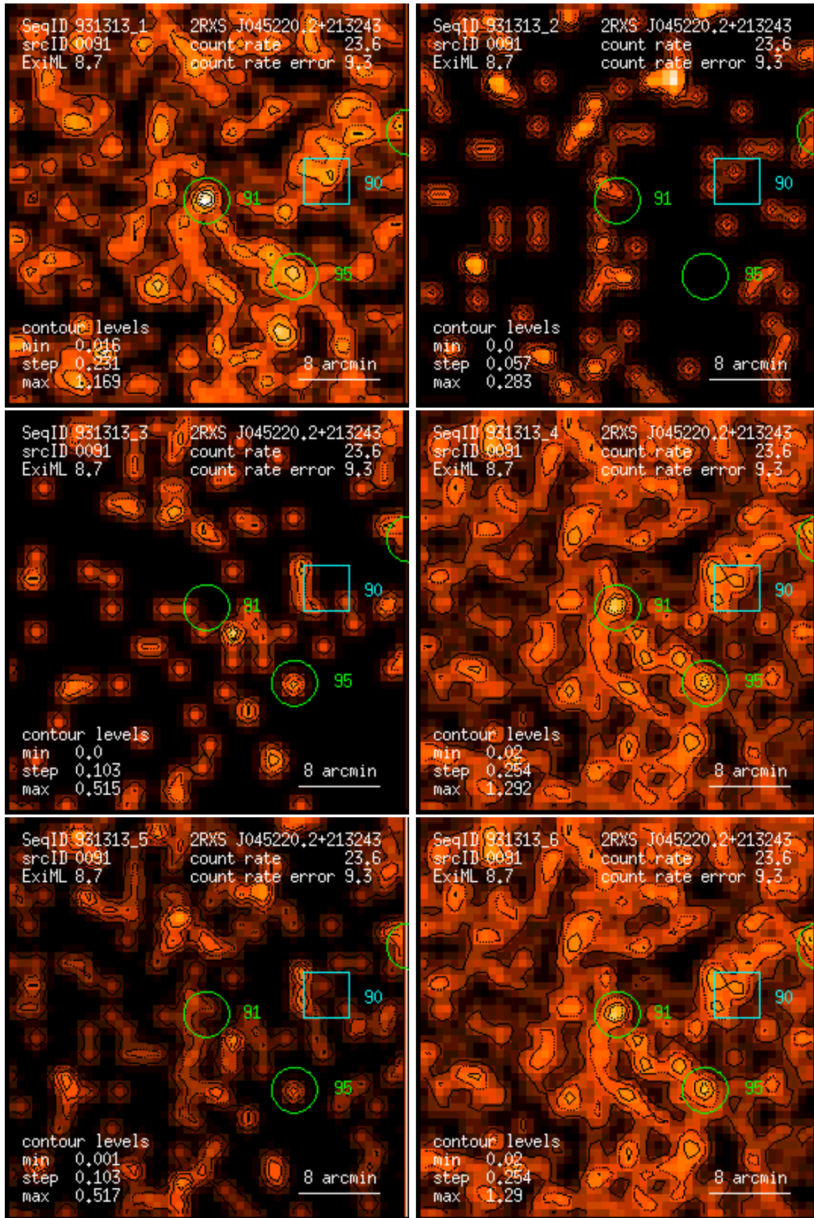
Figure 91: RASS 931313: detection 0091: band rate images, Gaussian filter: (1) PSPC channels 11 – 41, (2) 52 – 90, (3) 91 – 201, (4) 11 – 235, (5) 52 – 201, (6) 11 – 201. Broad band rates in counts/ks. Band rate contour levels in counts/ks/arcmin 2 .
