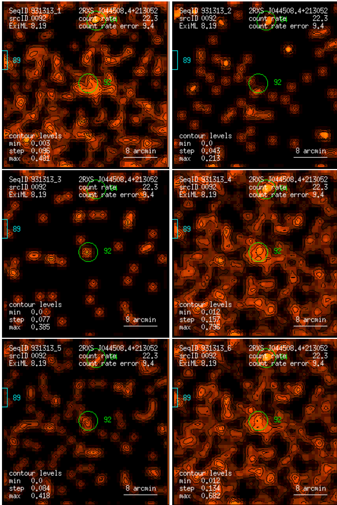
Figure 92: RASS 931313: detection 0092: band rate images, Gaussian filter: (1) PSPC channels 11 – 41, (2) 52 – 90, (3) 91 – 201, (4) 11 – 235, (5) 52 – 201, (6) 11 – 201. Broad band rates in counts/ks. Band rate contour levels in counts/ks/arcmin 2 .
