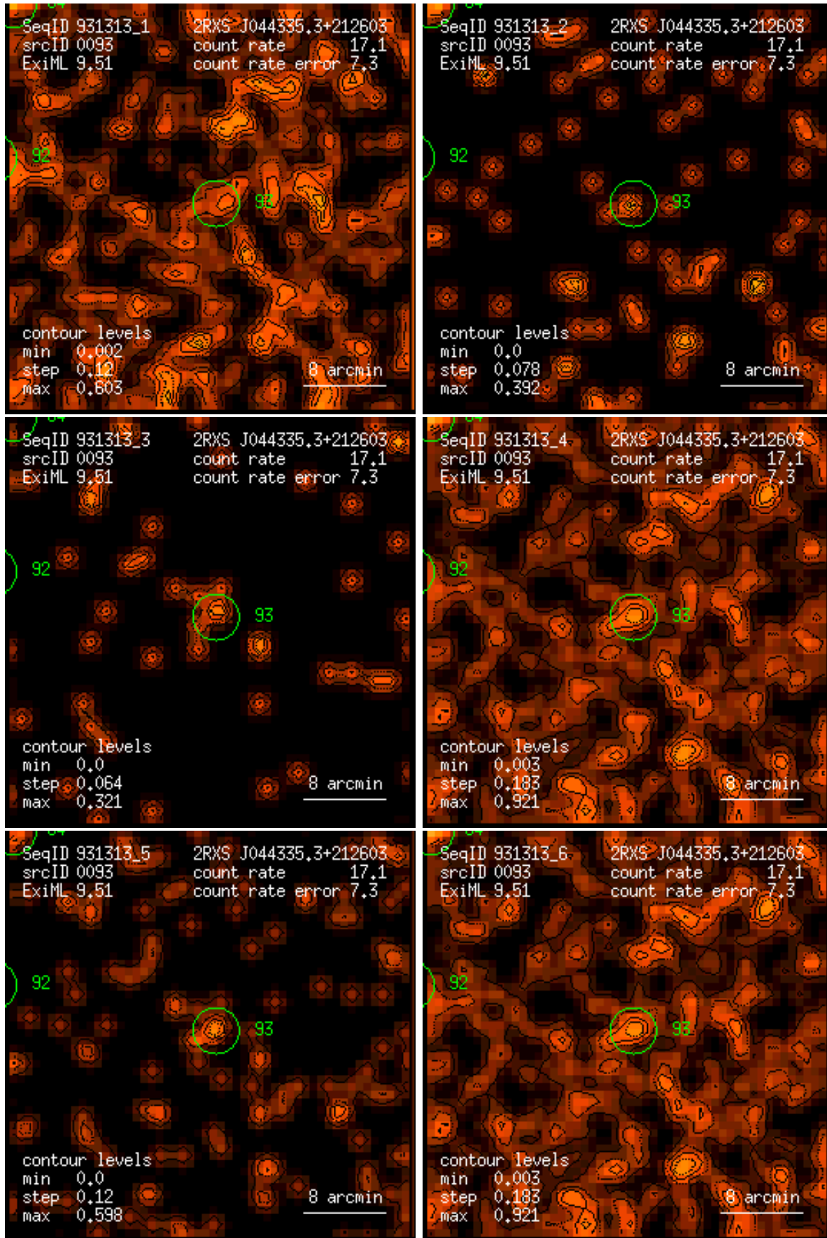
Figure 93: RASS 931313: detection 0093: band rate images, Gaussian filter: (1) PSPC channels 11 – 41, (2) 52 – 90, (3) 91 – 201, (4) 11 – 235, (5) 52 – 201, (6) 11 – 201. Broad band rates in counts/ks. Band rate contour levels in counts/ks/arcmin 2 .
