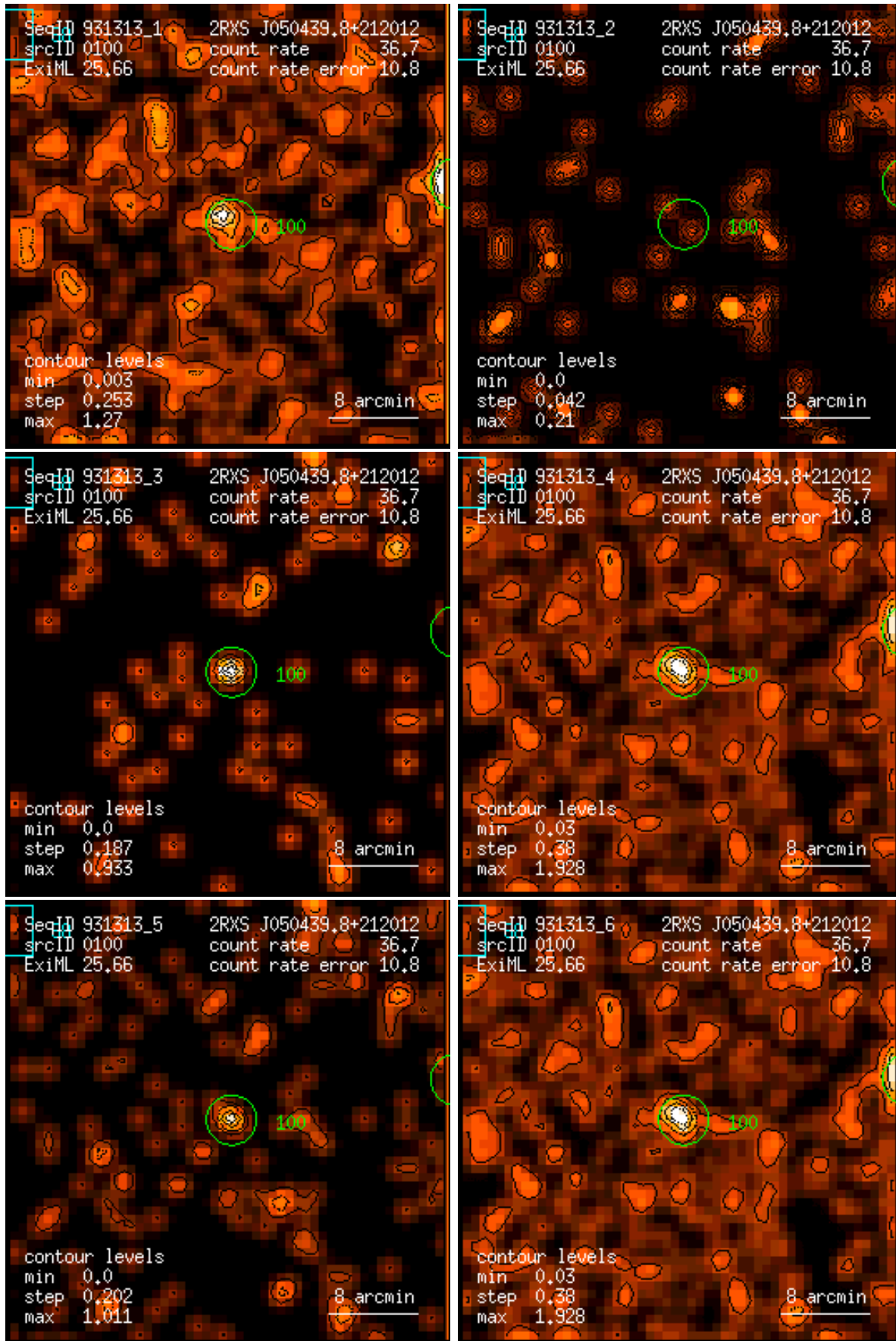
Figure 100: RASS 931313: detection 0100: band rate images, Gaussian filter: (1) PSPC channels 11 – 41, (2) 52 – 90, (3) 91 – 201, (4) 11 – 235, (5) 52 – 201, (6) 11 – 201. Broad band rates in counts/ks. Band rate contour levels in counts/ks/arcmin 2 .
