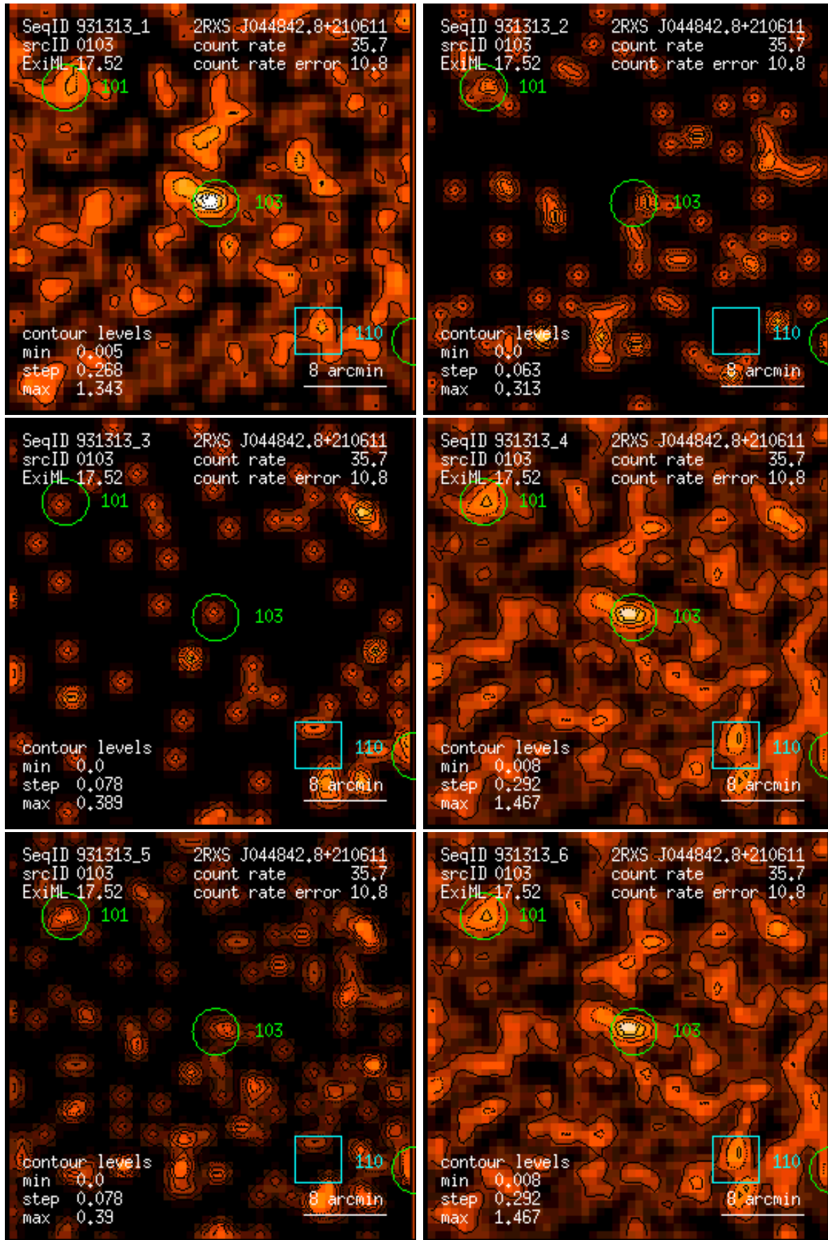
Figure 103: RASS 931313: detection 0103: band rate images, Gaussian filter: (1) PSPC channels 11 – 41, (2) 52 – 90, (3) 91 – 201, (4) 11 – 235, (5) 52 – 201, (6) 11 – 201. Broad band rates in counts/ks. Band rate contour levels in counts/ks/arcmin 2 .
