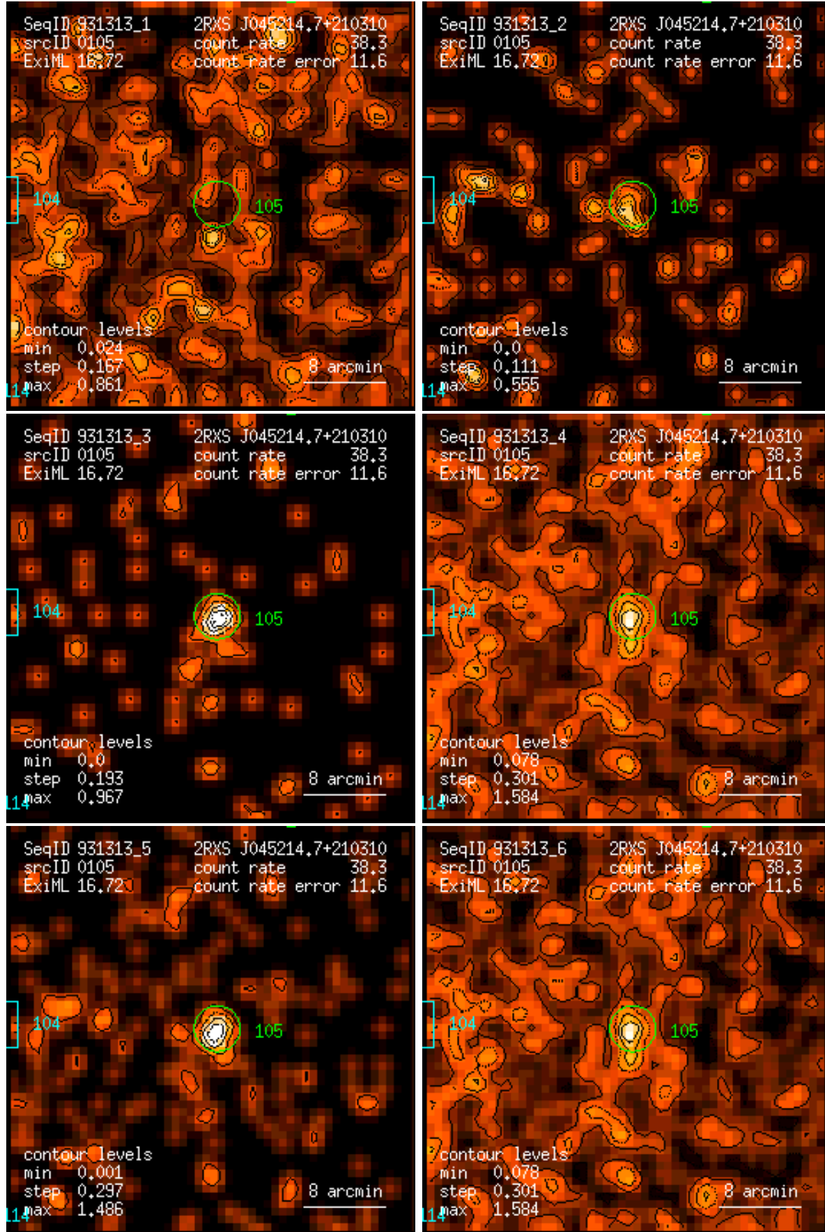
Figure 105: RASS 931313: detection 0105: band rate images, Gaussian filter: (1) PSPC channels 11 – 41, (2) 52 – 90, (3) 91 – 201, (4) 11 – 235, (5) 52 – 201, (6) 11 – 201. Broad band rates in counts/ks. Band rate contour levels in counts/ks/arcmin 2 .
