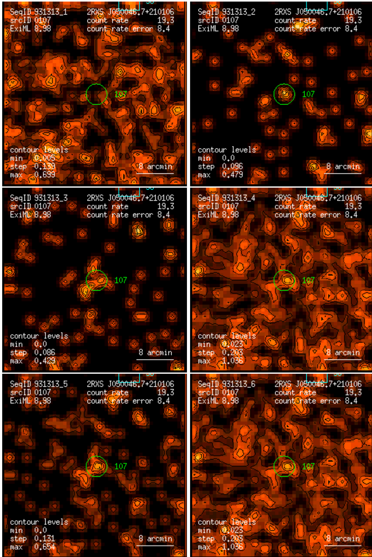
Figure 107: RASS 931313: detection 0107: band rate images, Gaussian filter: (1) PSPC channels 11 – 41, (2) 52 – 90, (3) 91 – 201, (4) 11 – 235, (5) 52 – 201, (6) 11 – 201. Broad band rates in counts/ks. Band rate contour levels in counts/ks/arcmin 2 .
