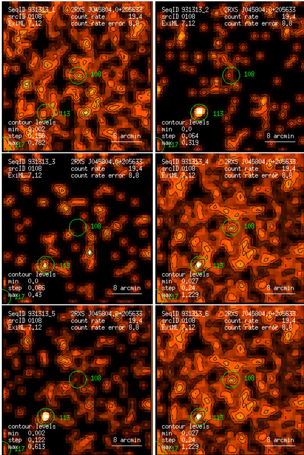
Figure 108: RASS 931313: detection 0108: band rate images, Gaussian filter: (1) PSPC channels 11 – 41, (2) 52 – 90, (3) 91 – 201, (4) 11 – 235, (5) 52 – 201, (6) 11 – 201. Broad band rates in counts/ks. Band rate contour levels in counts/ks/arcmin 2 .
