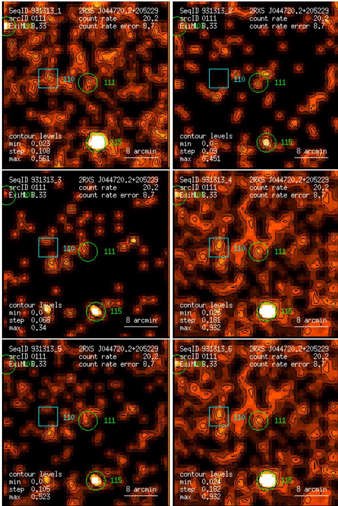
Figure 111: RASS 931313: detection 0111: band rate images, Gaussian filter: (1) PSPC channels 11 – 41, (2) 52 – 90, (3) 91 – 201, (4) 11 – 235, (5) 52 – 201, (6) 11 – 201. Broad band rates in counts/ks. Band rate contour levels in counts/ks/arcmin 2 .
