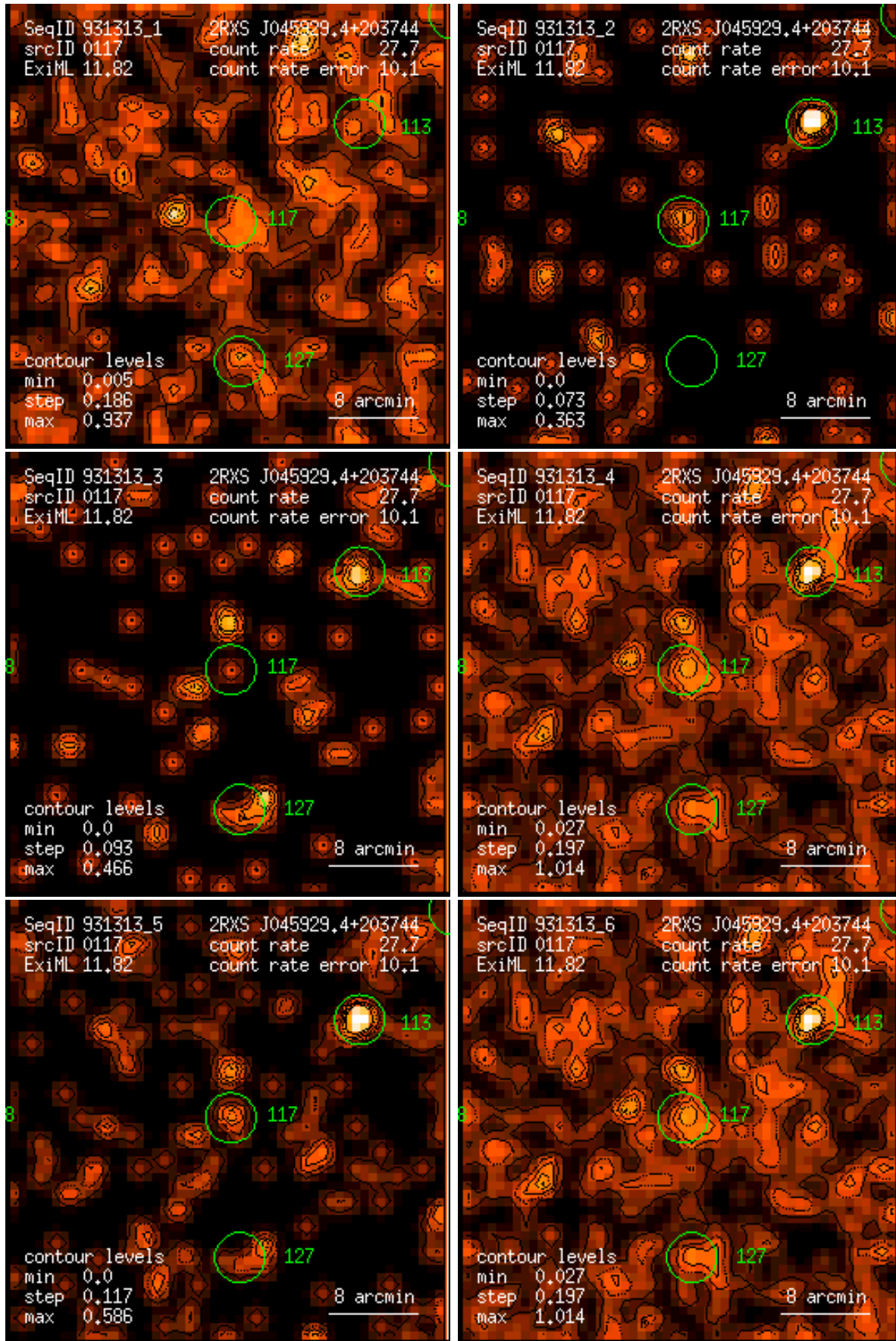
Figure 117: RASS 931313: detection 0117: band rate images, Gaussian filter: (1) PSPC channels 11 – 41, (2) 52 – 90, (3) 91 – 201, (4) 11 – 235, (5) 52 – 201, (6) 11 – 201. Broad band rates in counts/ks. Band rate contour levels in counts/ks/arcmin 2 .
