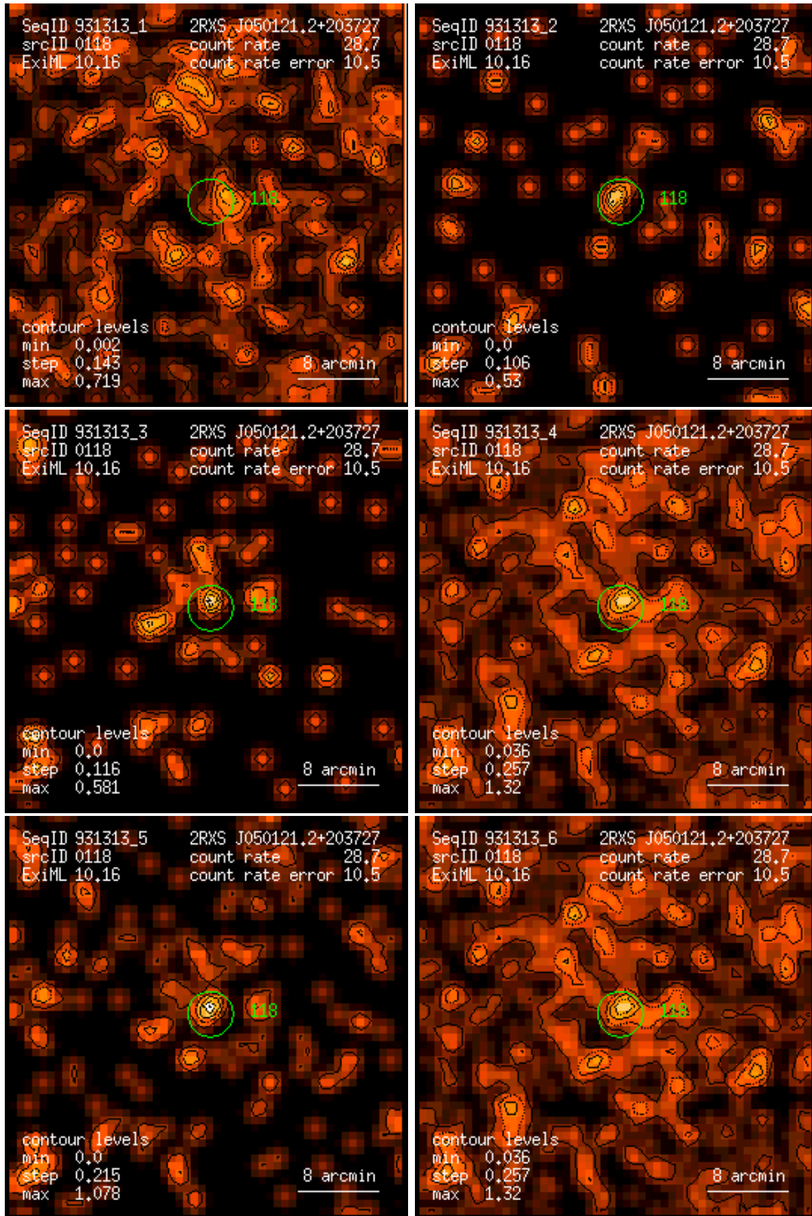
Figure 118: RASS 931313: detection 0118: band rate images, Gaussian filter: (1) PSPC channels 11 – 41, (2) 52 – 90, (3) 91 – 201, (4) 11 – 235, (5) 52 – 201, (6) 11 – 201. Broad band rates in counts/ks. Band rate contour levels in counts/ks/arcmin 2 .
