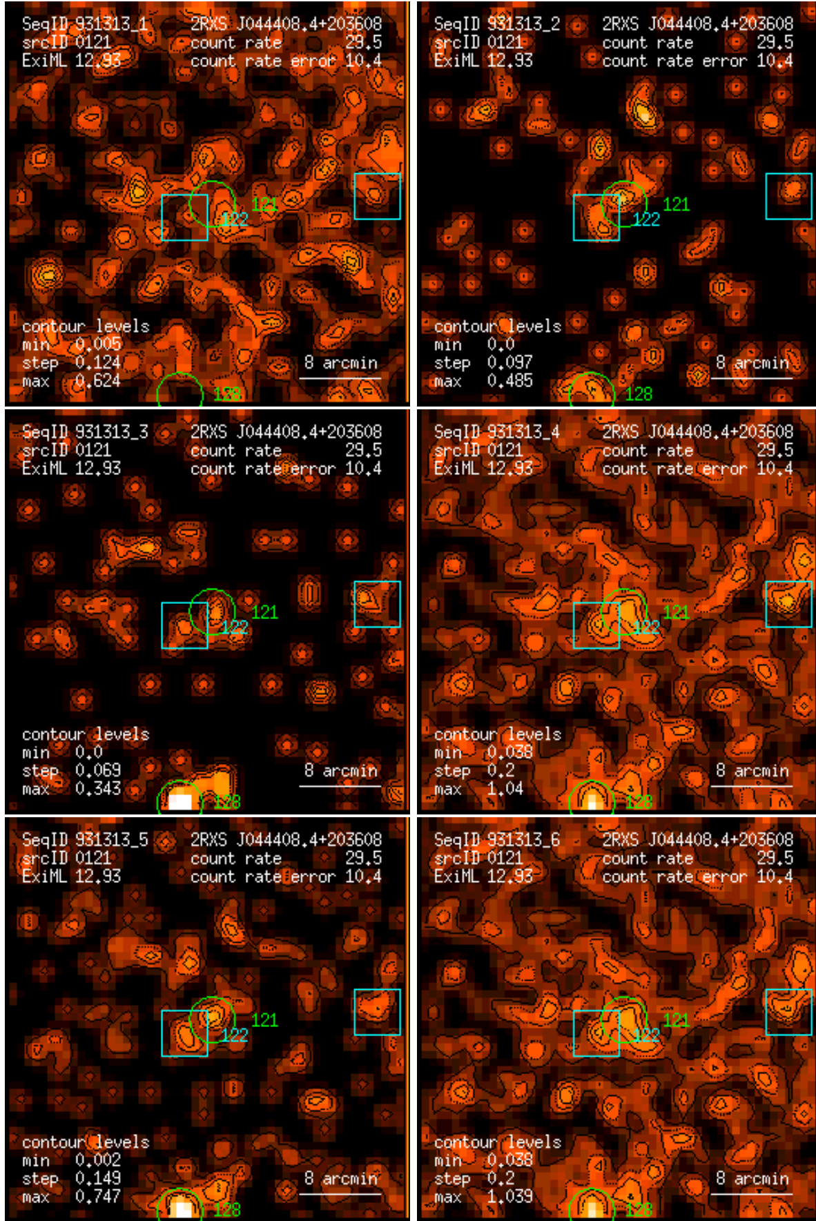
Figure 121: RASS 931313: detection 0121: band rate images, Gaussian filter: (1) PSPC channels 11 – 41, (2) 52 – 90, (3) 91 – 201, (4) 11 – 235, (5) 52 – 201, (6) 11 – 201. Broad band rates in counts/ks. Band rate contour levels in counts/ks/arcmin 2 .
