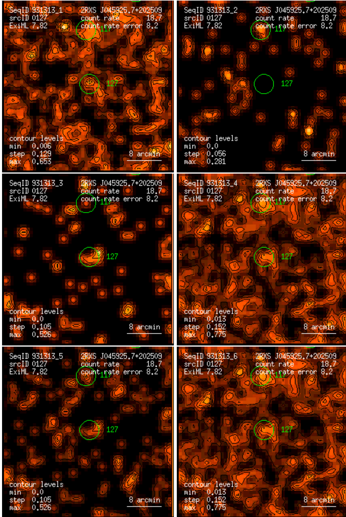
Figure 127: RASS 931313: detection 0127: band rate images, Gaussian filter: (1) PSPC channels 11 – 41, (2) 52 – 90, (3) 91 – 201, (4) 11 – 235, (5) 52 – 201, (6) 11 – 201. Broad band rates in counts/ks. Band rate contour levels in counts/ks/arcmin 2 .
