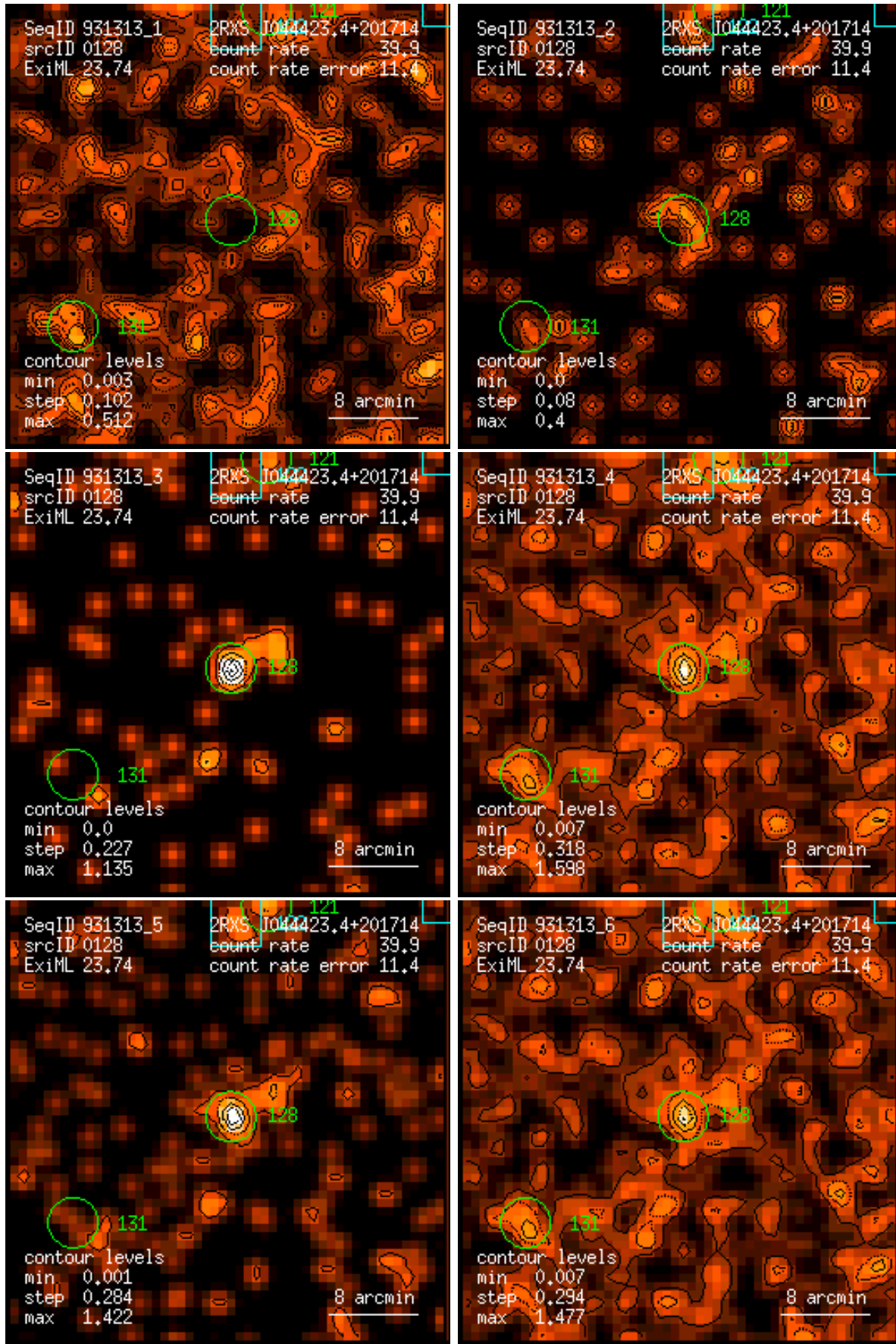
Figure 128: RASS 931313: detection 0128: band rate images, Gaussian filter: (1) PSPC channels 11 – 41, (2) 52 – 90, (3) 91 – 201, (4) 11 – 235, (5) 52 – 201, (6) 11 – 201. Broad band rates in counts/ks. Band rate contour levels in counts/ks/arcmin 2 .
