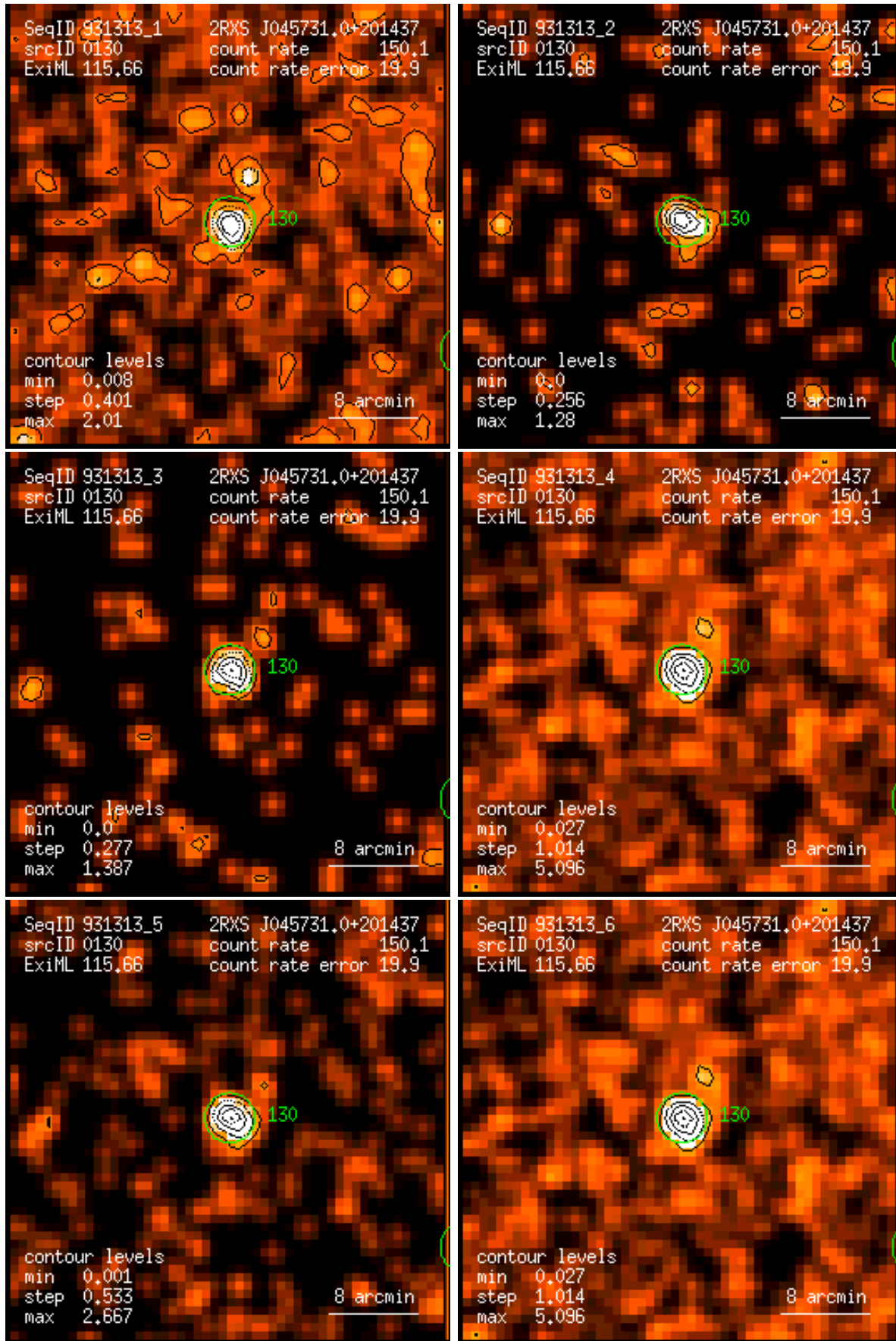
Figure 130: RASS 931313: detection 0130: band rate images, Gaussian filter: (1) PSPC channels 11 – 41, (2) 52 – 90, (3) 91 – 201, (4) 11 – 235, (5) 52 – 201, (6) 11 – 201. Broad band rates in counts/ks. Band rate contour levels in counts/ks/arcmin 2 .
