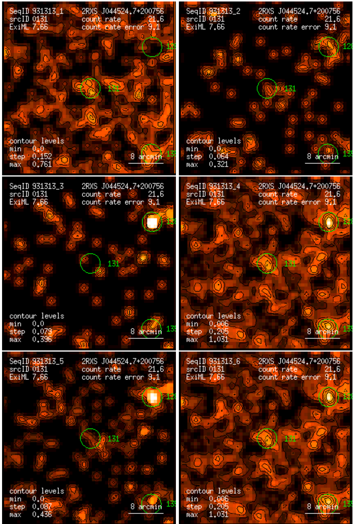
Figure 131: RASS 931313: detection 0131: band rate images, Gaussian filter: (1) PSPC channels 11 – 41, (2) 52 – 90, (3) 91 – 201, (4) 11 – 235, (5) 52 – 201, (6) 11 – 201. Broad band rates in counts/ks. Band rate contour levels in counts/ks/arcmin 2 .
