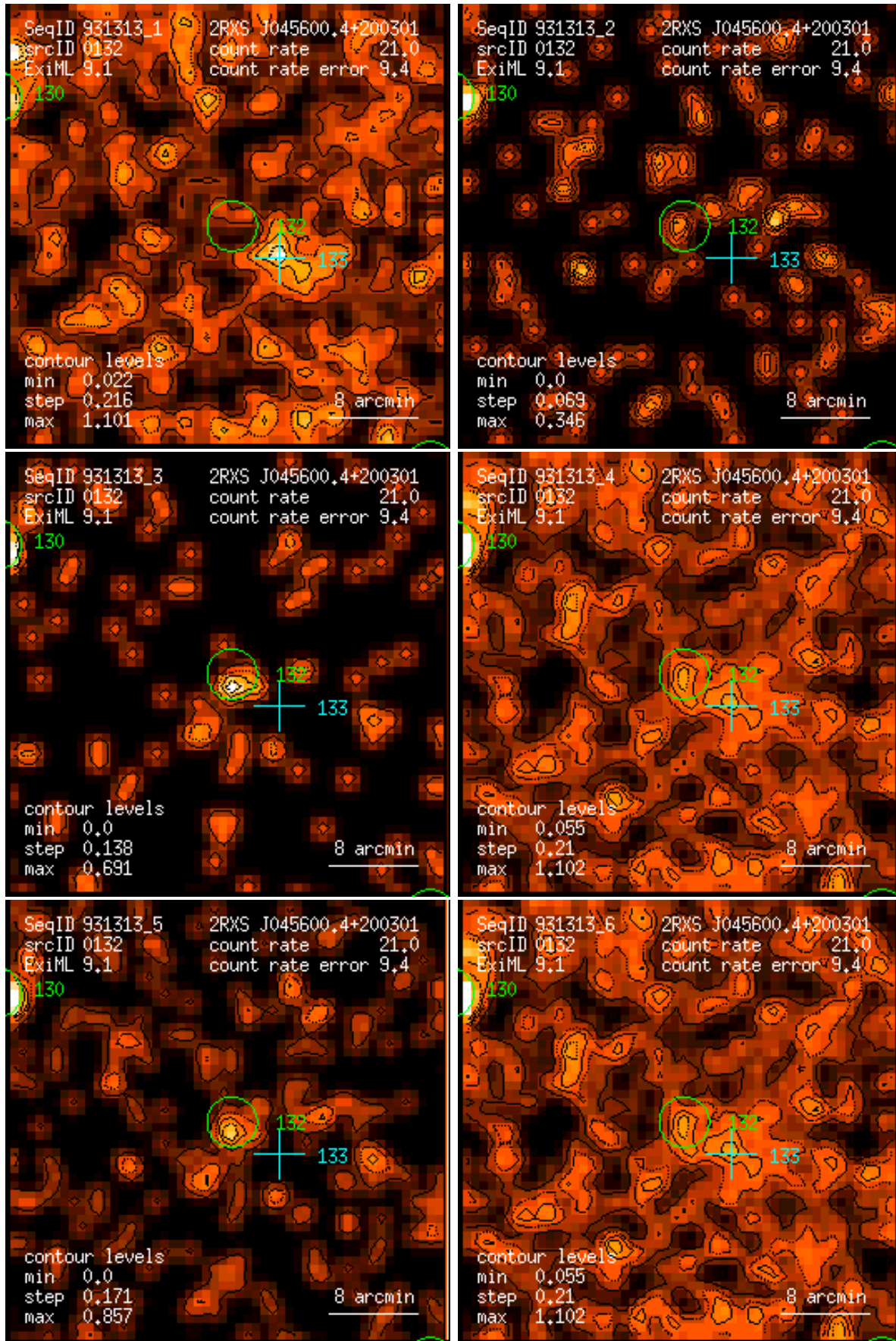
Figure 132: RASS 931313: detection 0132: band rate images, Gaussian filter: (1) PSPC channels 11 – 41, (2) 52 – 90, (3) 91 – 201, (4) 11 – 235, (5) 52 – 201, (6) 11 – 201. Broad band rates in counts/ks. Band rate contour levels in counts/ks/arcmin 2 .
