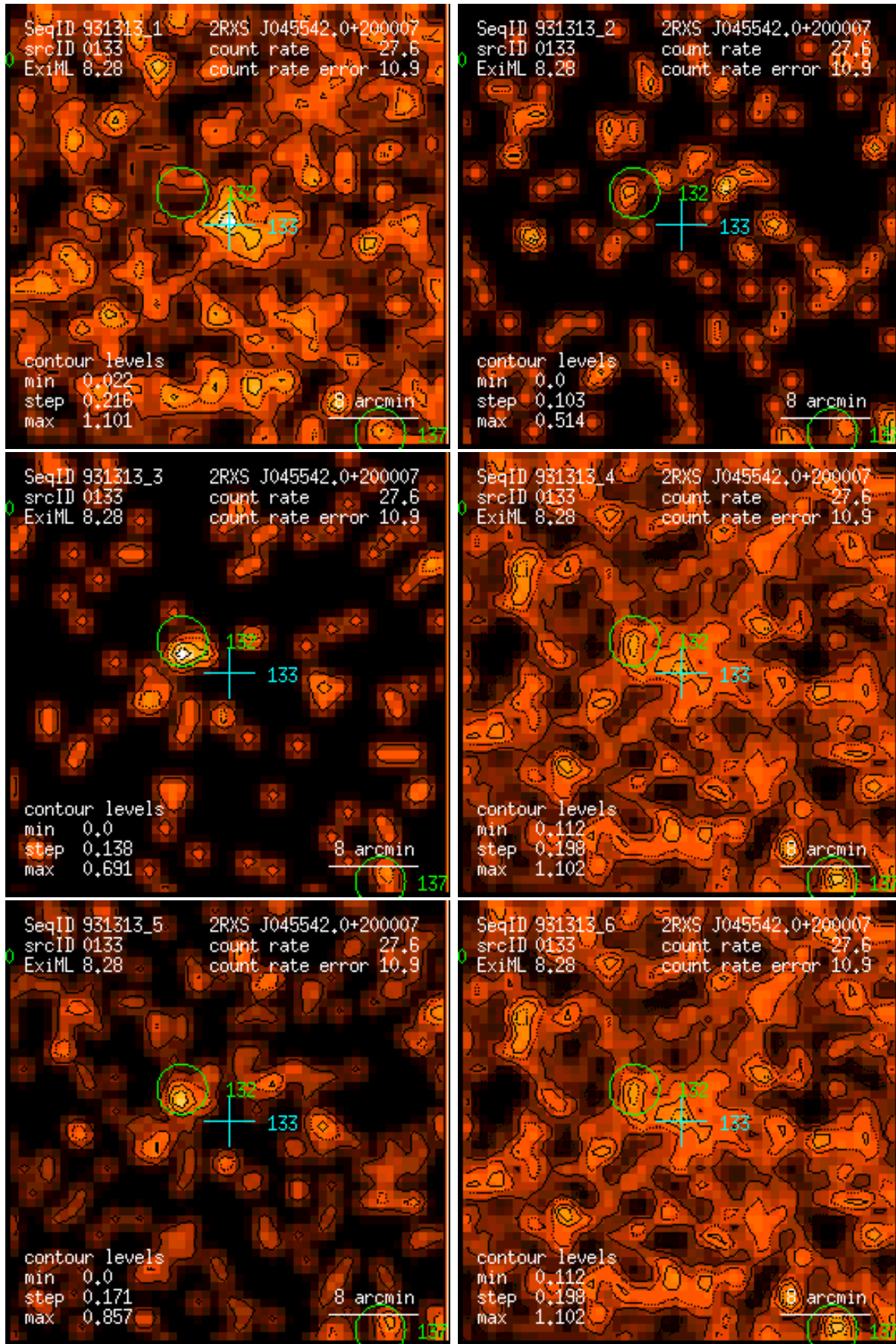
Figure 133: RASS 931313: detection 0133: band rate images, Gaussian filter: (1) PSPC channels 11 – 41, (2) 52 – 90, (3) 91 – 201, (4) 11 – 235, (5) 52 – 201, (6) 11 – 201. Broad band rates in counts/ks. Band rate contour levels in counts/ks/arcmin 2 .
