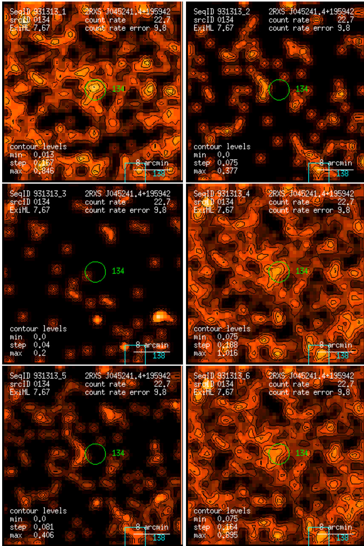
Figure 134: RASS 931313: detection 0134: band rate images, Gaussian filter: (1) PSPC channels 11 – 41, (2) 52 – 90, (3) 91 – 201, (4) 11 – 235, (5) 52 – 201, (6) 11 – 201. Broad band rates in counts/ks. Band rate contour levels in counts/ks/arcmin 2 .
