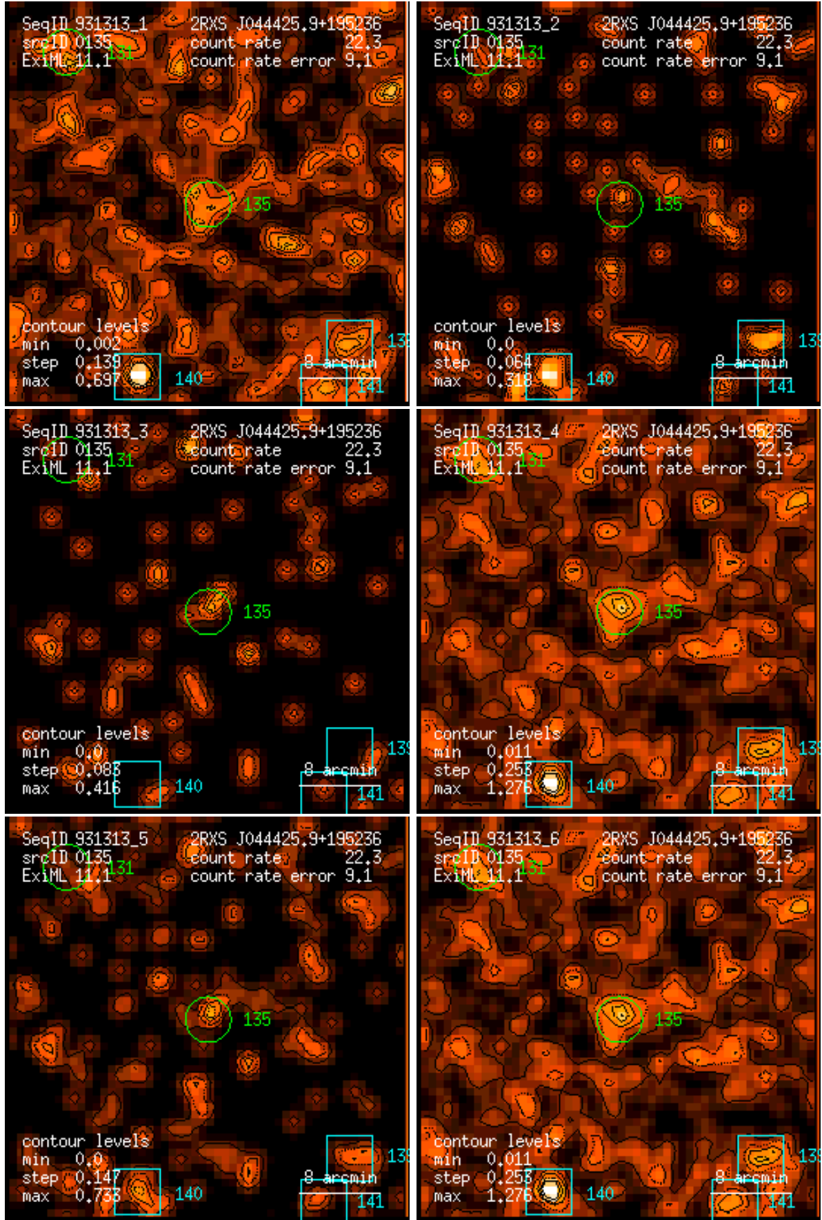
Figure 135: RASS 931313: detection 0135: band rate images, Gaussian filter: (1) PSPC channels 11 – 41, (2) 52 – 90, (3) 91 – 201, (4) 11 – 235, (5) 52 – 201, (6) 11 – 201. Broad band rates in counts/ks. Band rate contour levels in counts/ks/arcmin 2 .
