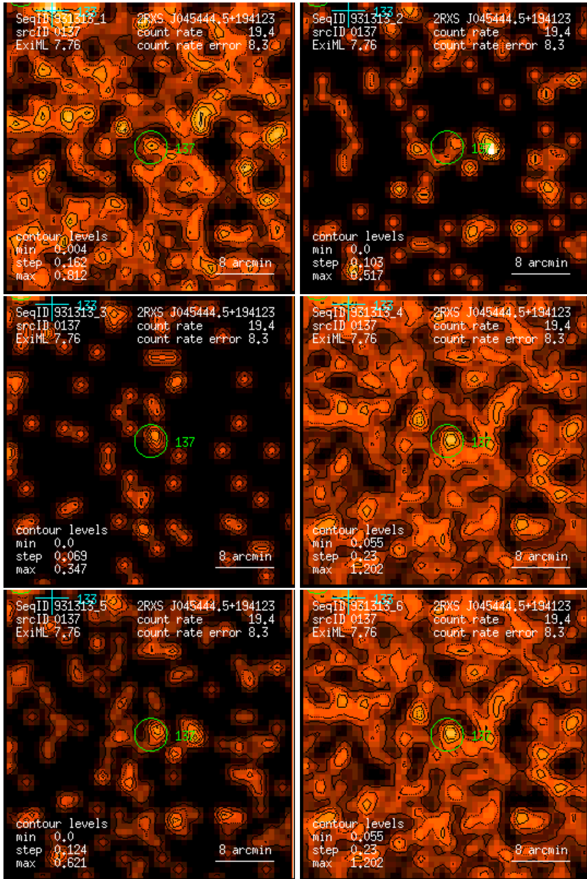
Figure 137: RASS 931313: detection 0137: band rate images, Gaussian filter: (1) PSPC channels 11 – 41, (2) 52 – 90, (3) 91 – 201, (4) 11 – 235, (5) 52 – 201, (6) 11 – 201. Broad band rates in counts/ks. Band rate contour levels in counts/ks/arcmin 2 .
