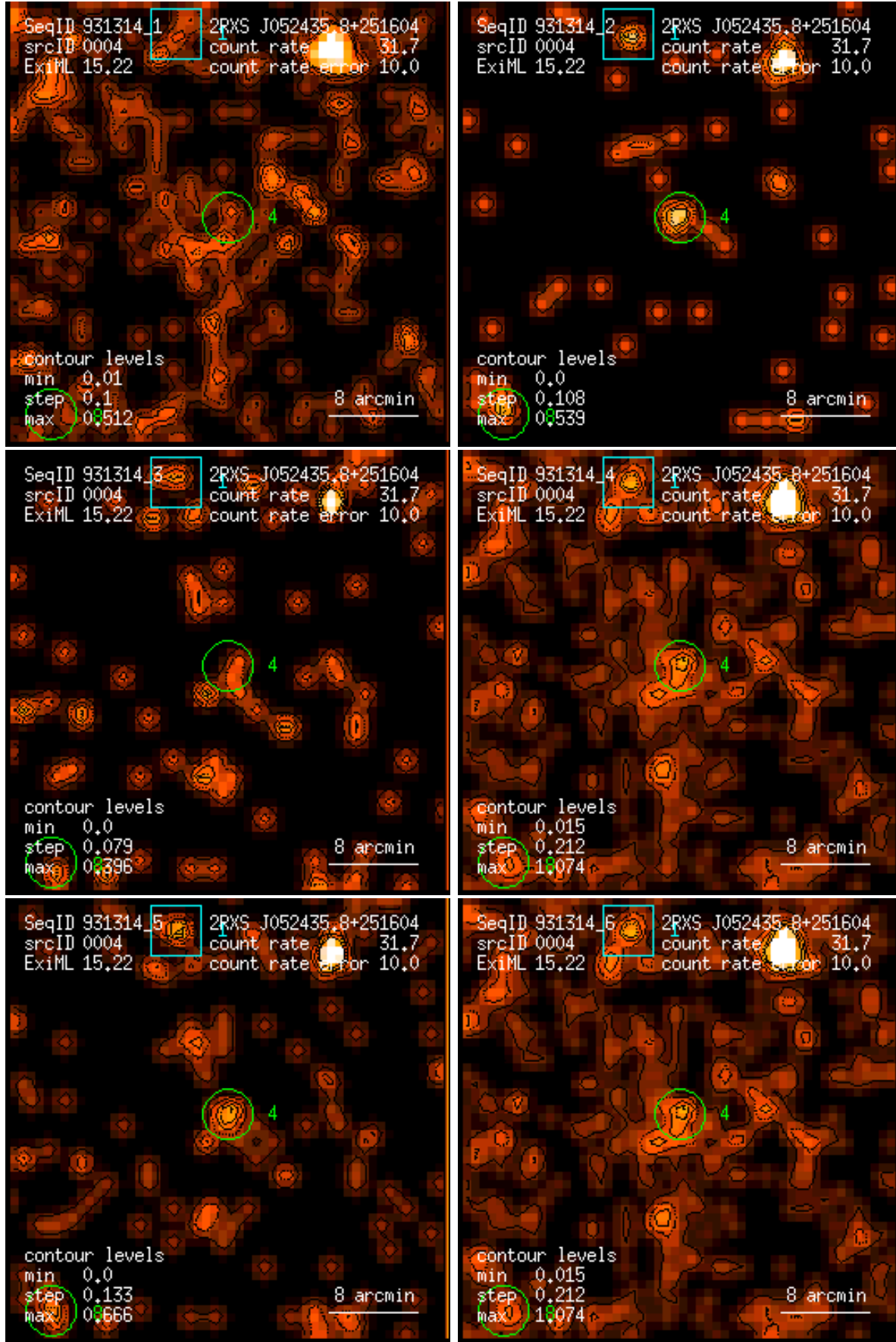
Figure 4: RASS 931314: detection 0004: band rate images, Gaussian filter: (1) PSPC channels 11 – 41, (2) 52 – 90, (3) 91 – 201, (4) 11 – 235, (5) 52 – 201, (6) 11 – 201. Broad band rates in counts/ks. Band rate contour levels in counts/ks/arcmin 2 .
