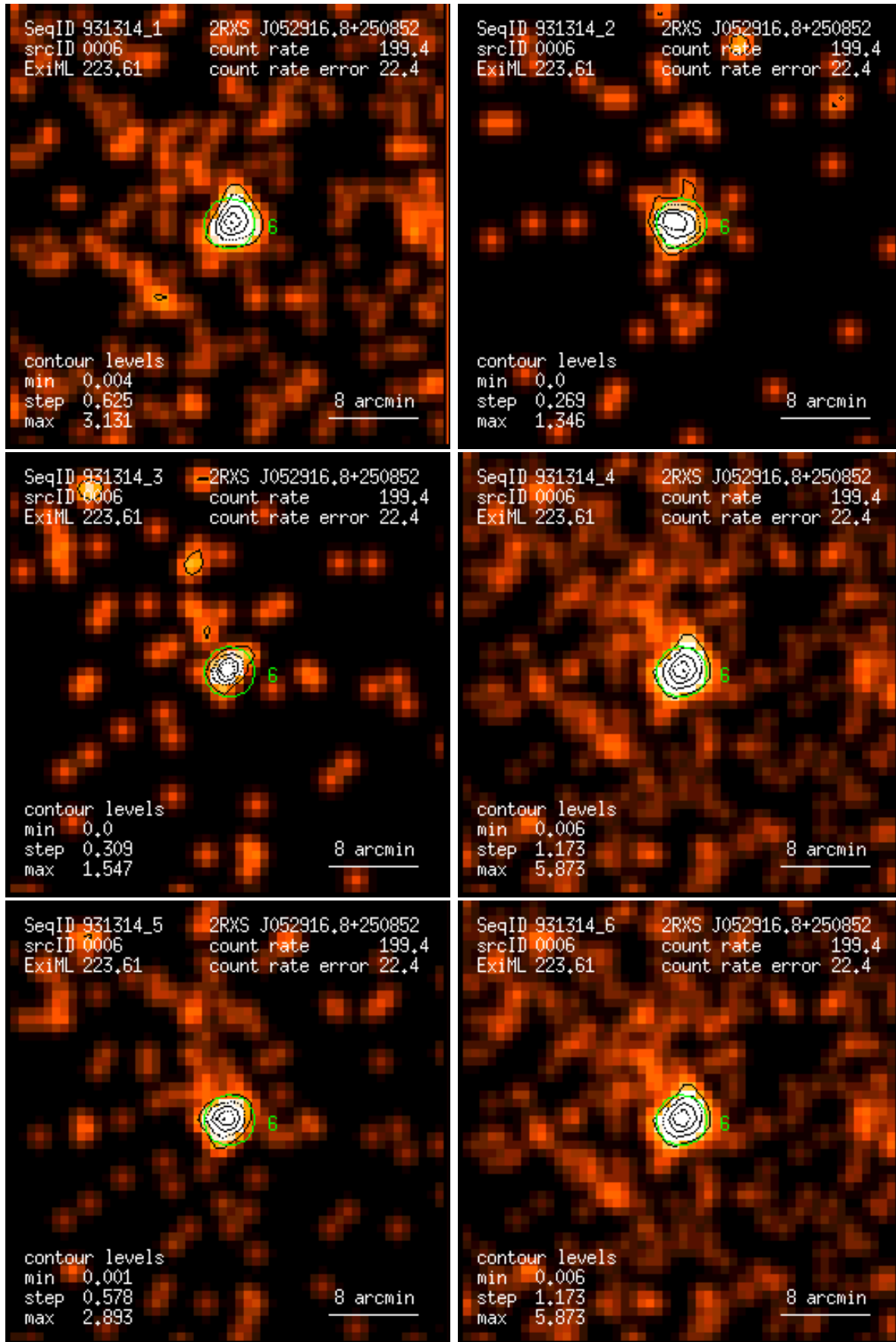
Figure 6: RASS 931314: detection 0006: band rate images, Gaussian filter: (1) PSPC channels 11 – 41, (2) 52 – 90, (3) 91 – 201, (4) 11 – 235, (5) 52 – 201, (6) 11 – 201. Broad band rates in counts/ks. Band rate contour levels in counts/ks/arcmin 2 .
