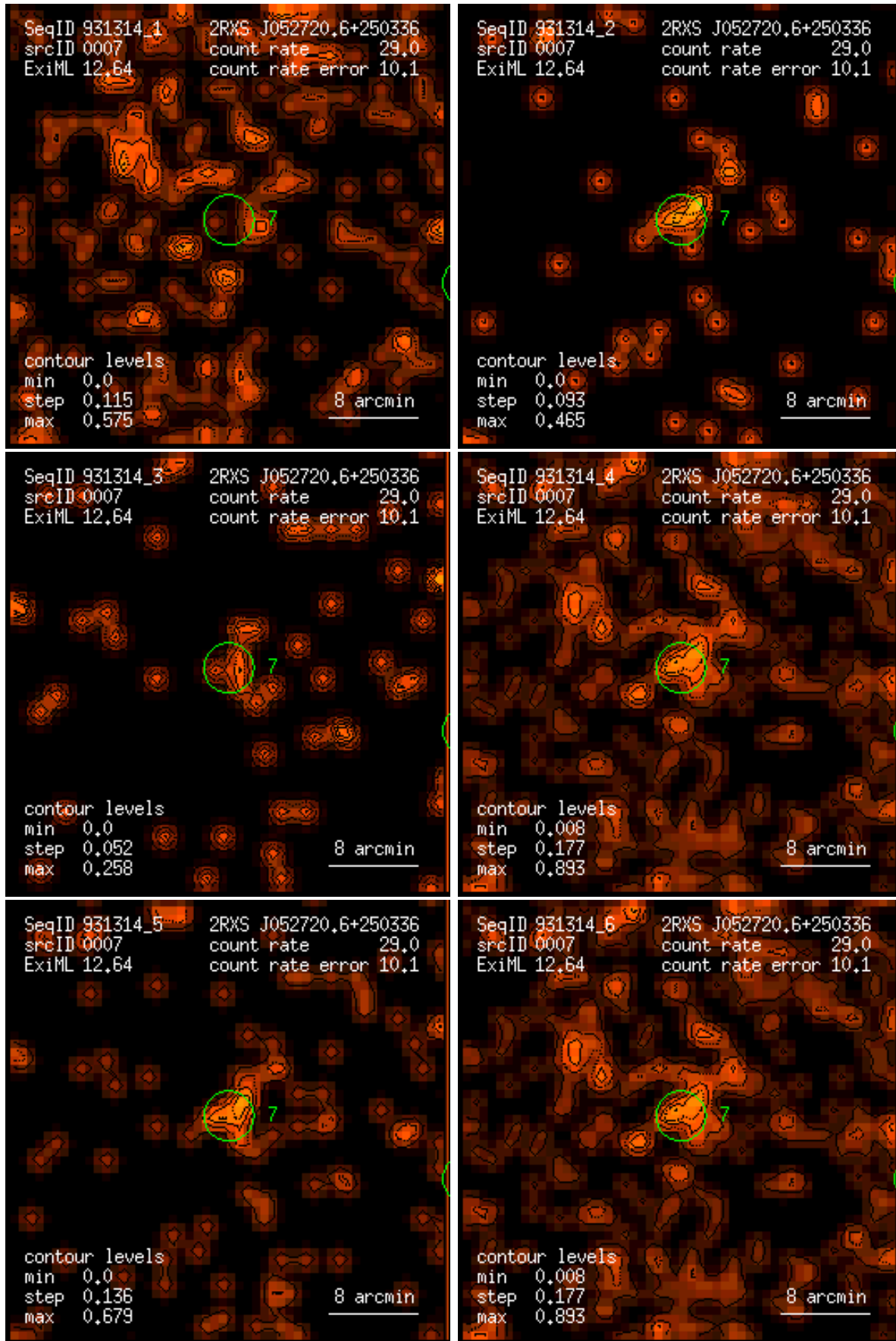
Figure 7: RASS 931314: detection 0007: band rate images, Gaussian filter: (1) PSPC channels 11 – 41, (2) 52 – 90, (3) 91 – 201, (4) 11 – 235, (5) 52 – 201, (6) 11 – 201. Broad band rates in counts/ks. Band rate contour levels in counts/ks/arcmin 2 .
