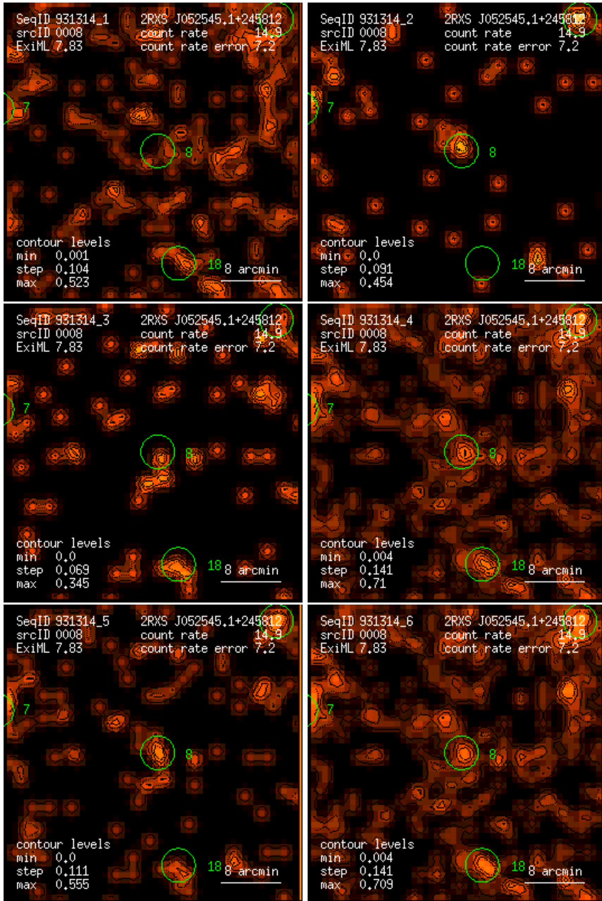
Figure 8: RASS 931314: detection 0008: band rate images, Gaussian filter: (1) PSPC channels 11 – 41, (2) 52 – 90, (3) 91 – 201, (4) 11 – 235, (5) 52 – 201, (6) 11 – 201. Broad band rates in counts/ks. Band rate contour levels in counts/ks/arcmin 2 .
